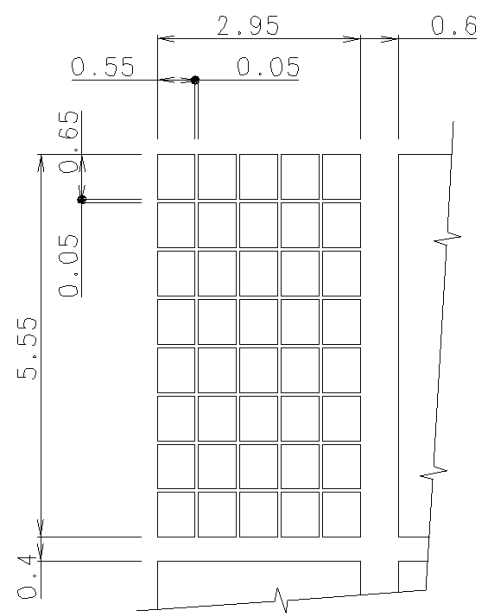
DOT DETAIL SCALE 10/1
