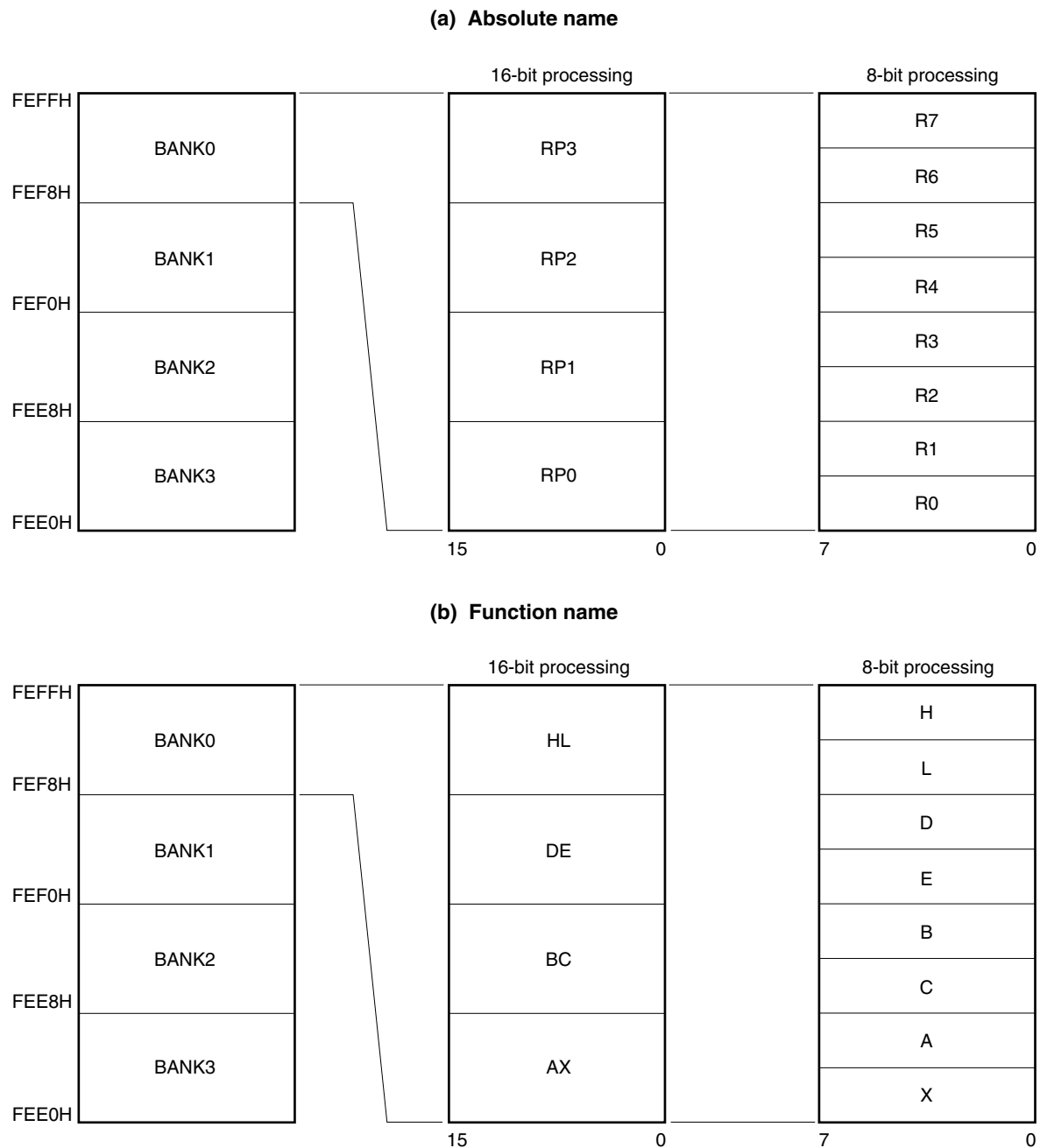
Figure 3-15. Configuration of General-Purpose Registers
