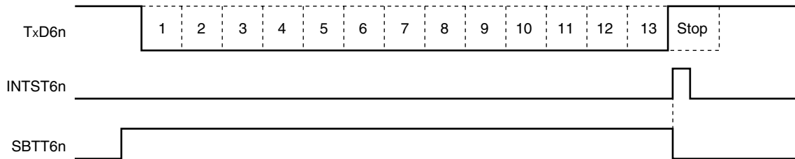
Figure 14-30. SBF Transmission
