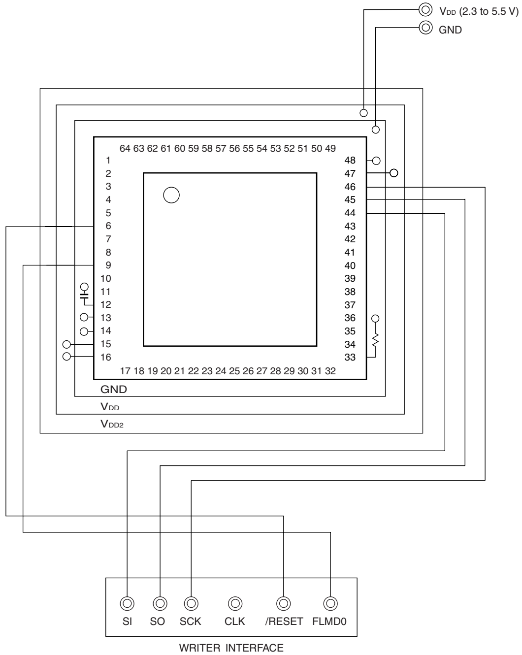
Figure 24-3. Example of Wiring Adapter for Flash Memory Writing in 3-Wire Serial I/O (CS110) Mode
