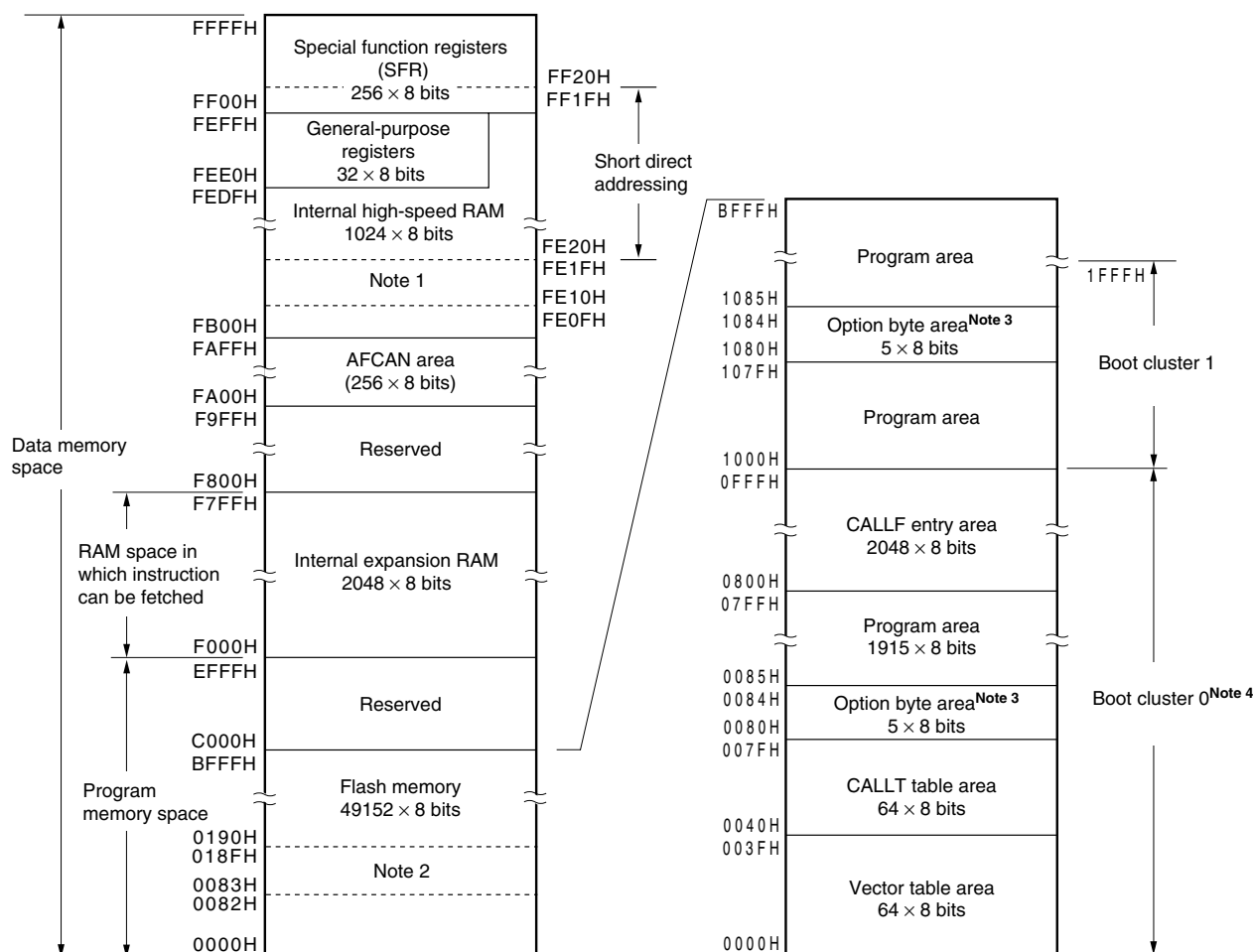
Figure 3-1. Memory Map ( \mu PD78F0887)
