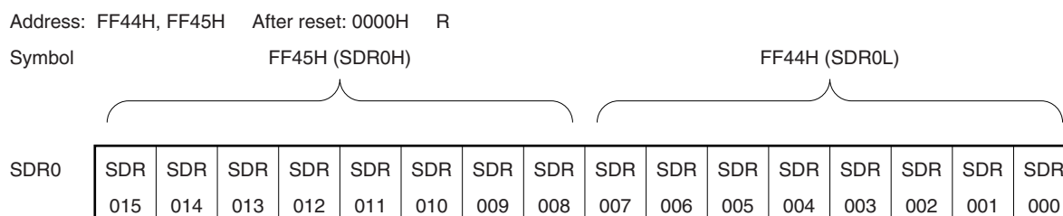
Figure 20-2. Format of Remainder Data Register 0 (SDR0)
