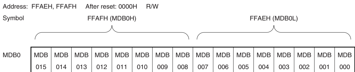
Figure 20-4. Format of Multiplication/Division Data Register B0 (MDB0)
