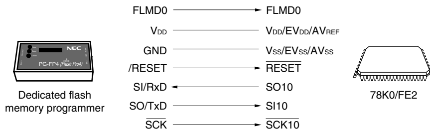
Figure 24-6. Communication with Dedicated Flash Memory Programmer (CSI10)
