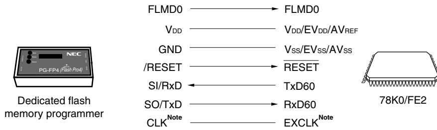
Figure 24-7. Communication with Dedicated Flash Memory Programmer (UART60)
