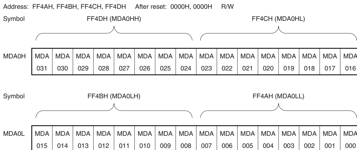
Figure 20-3. Format of Multiplication/Division Data Register A0 (MDA0H, MDA0L)
