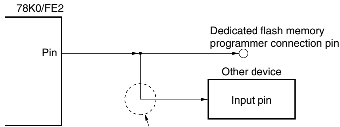
Figure 24-10. Malfunction of Other Device
