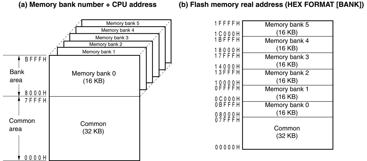
Figure 4-2. Address View
