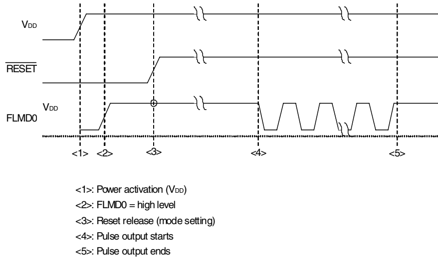
Figure 1-4. Setting Flash Memory Programming Mode and Selecting Communication Mode
