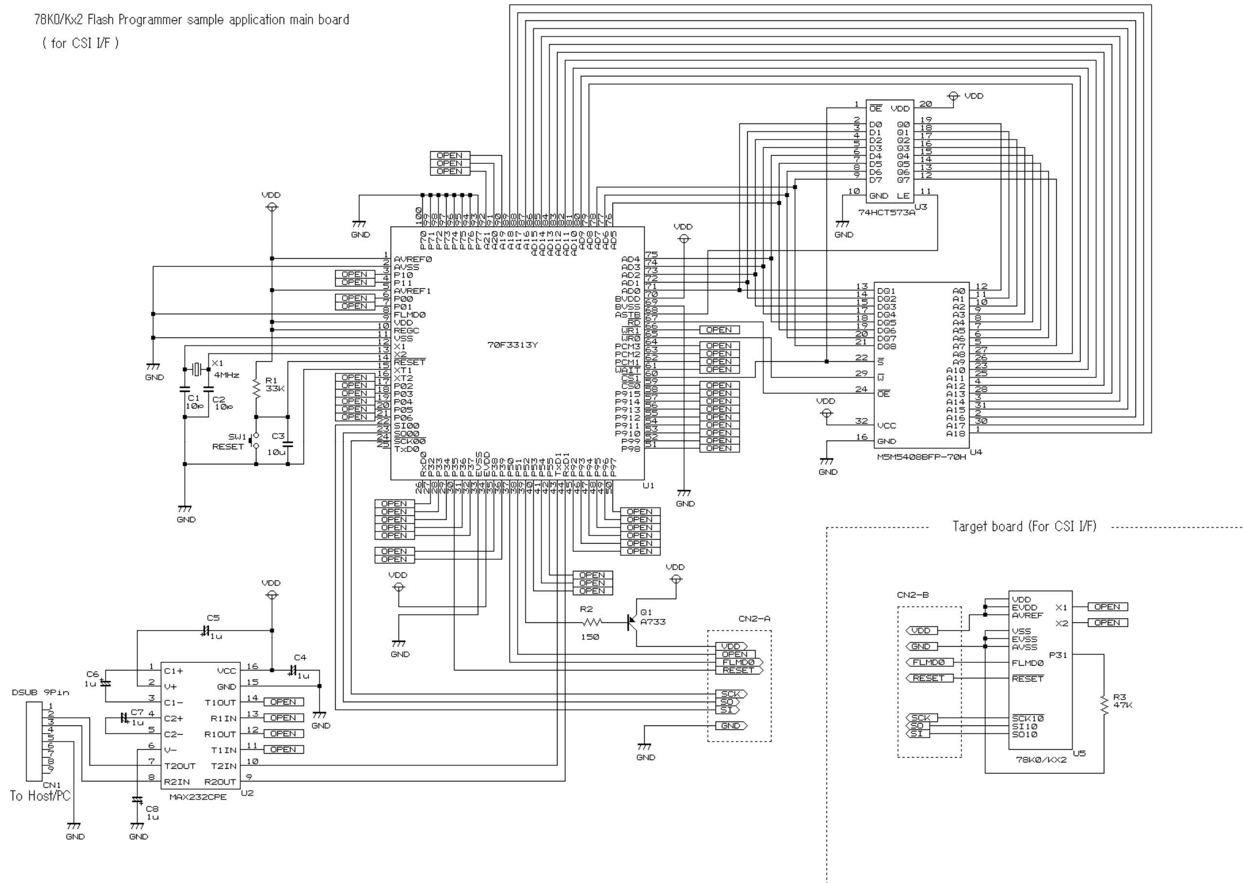
Figure A-3. Reference Circuit Diagram of Programmer and 78K0/Kx2 (During CSI Communication)
