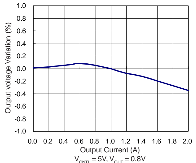
Output Voltage Load Regulation
