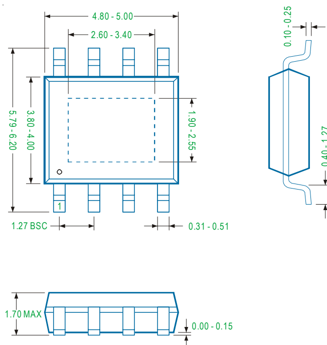
PSOP-8L
