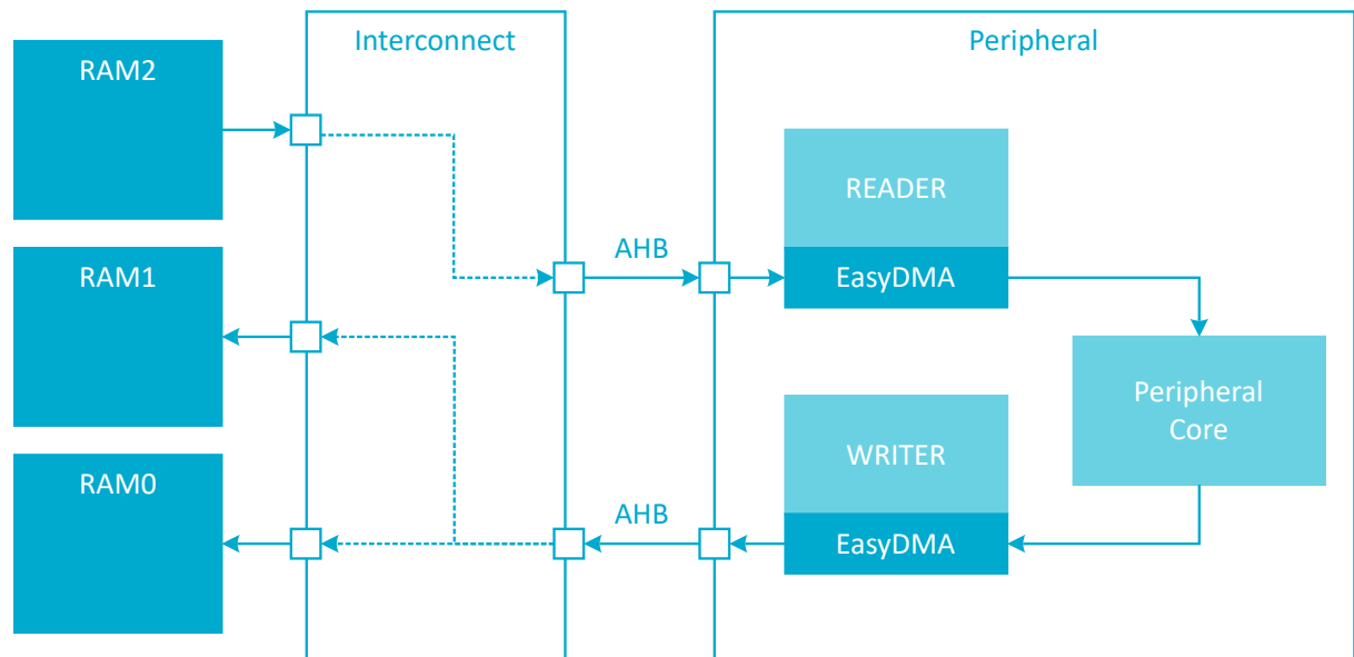
Figure 5: EasyDMA example
