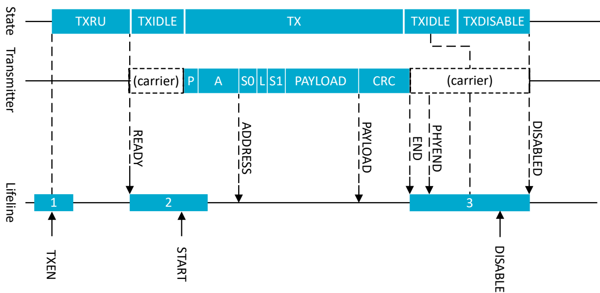
Figure 115: Transmit sequence
