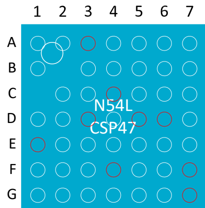
Figure 172: CSP47 pin assignments, top view
