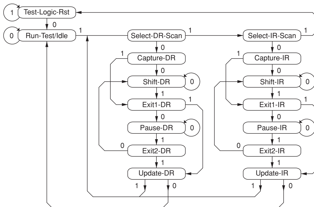
Figure 19. TAP States
