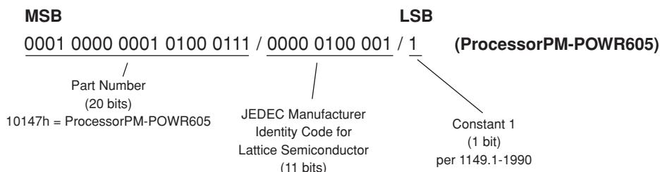
Figure 20. ProcessorPM-POWR605 ID Code
