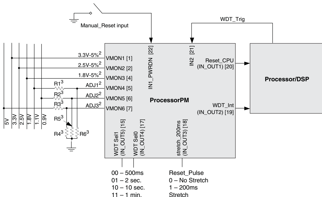
Figure 17. Reset Generator Programmable Pulse Stretch and Watchdog Timer Programmable Up to One Minute (Initial Factory Configuration) 1
