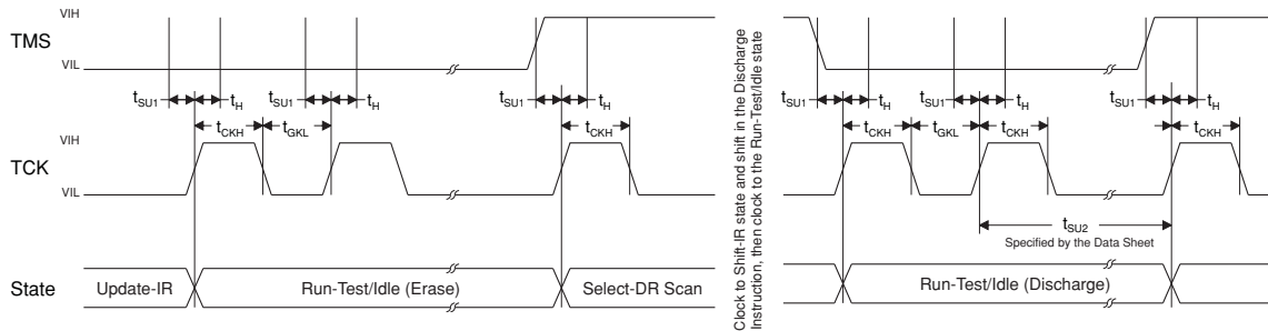
Figure 6. Programming Timing Diagram
