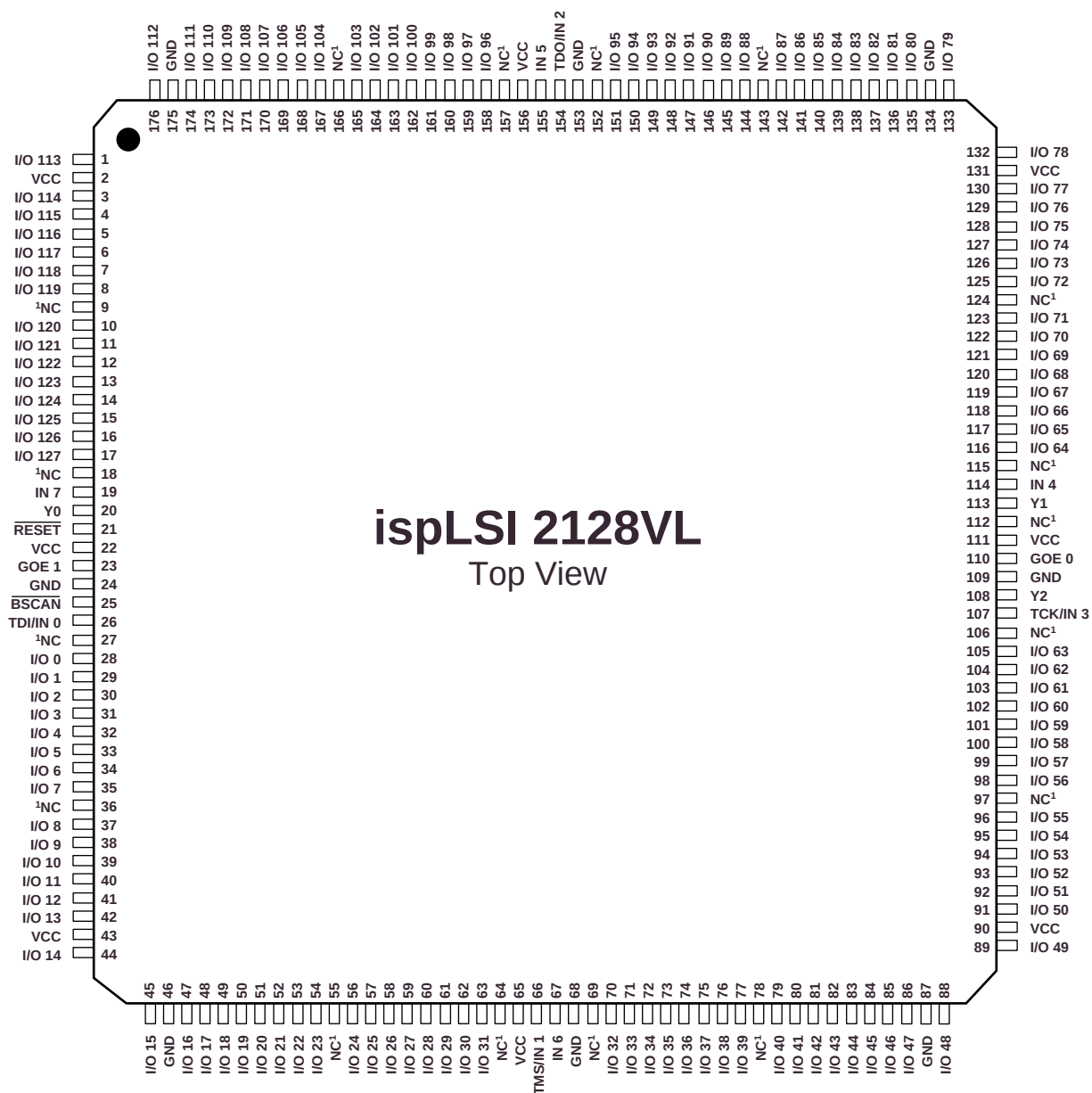
ispLSI 2128VL 176-Pin TQFP Pinout Diagram
