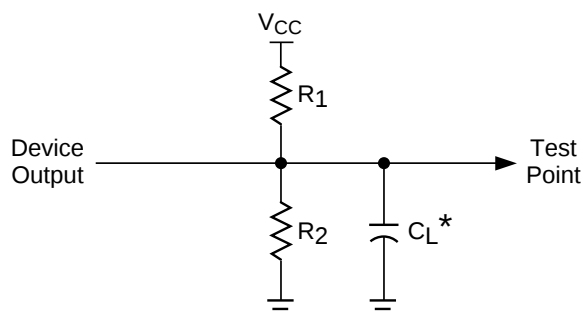
Figure 2. Test Load
