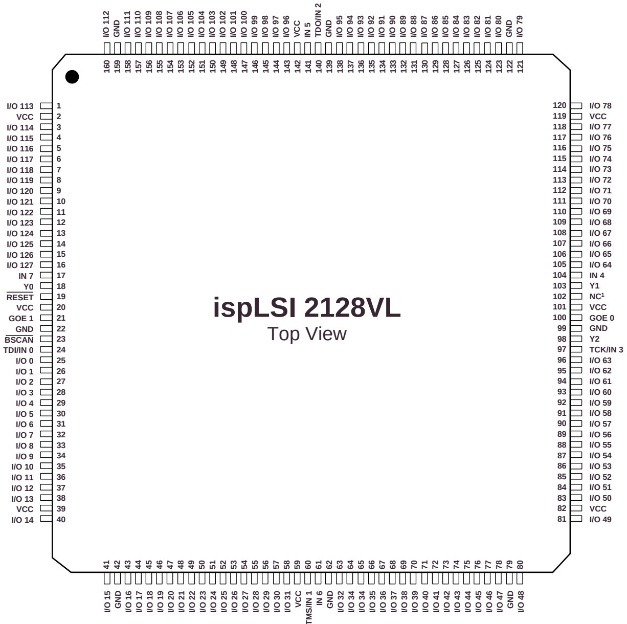
ispLSI 2128VL 160-Pin PQFP Pinout Diagram
