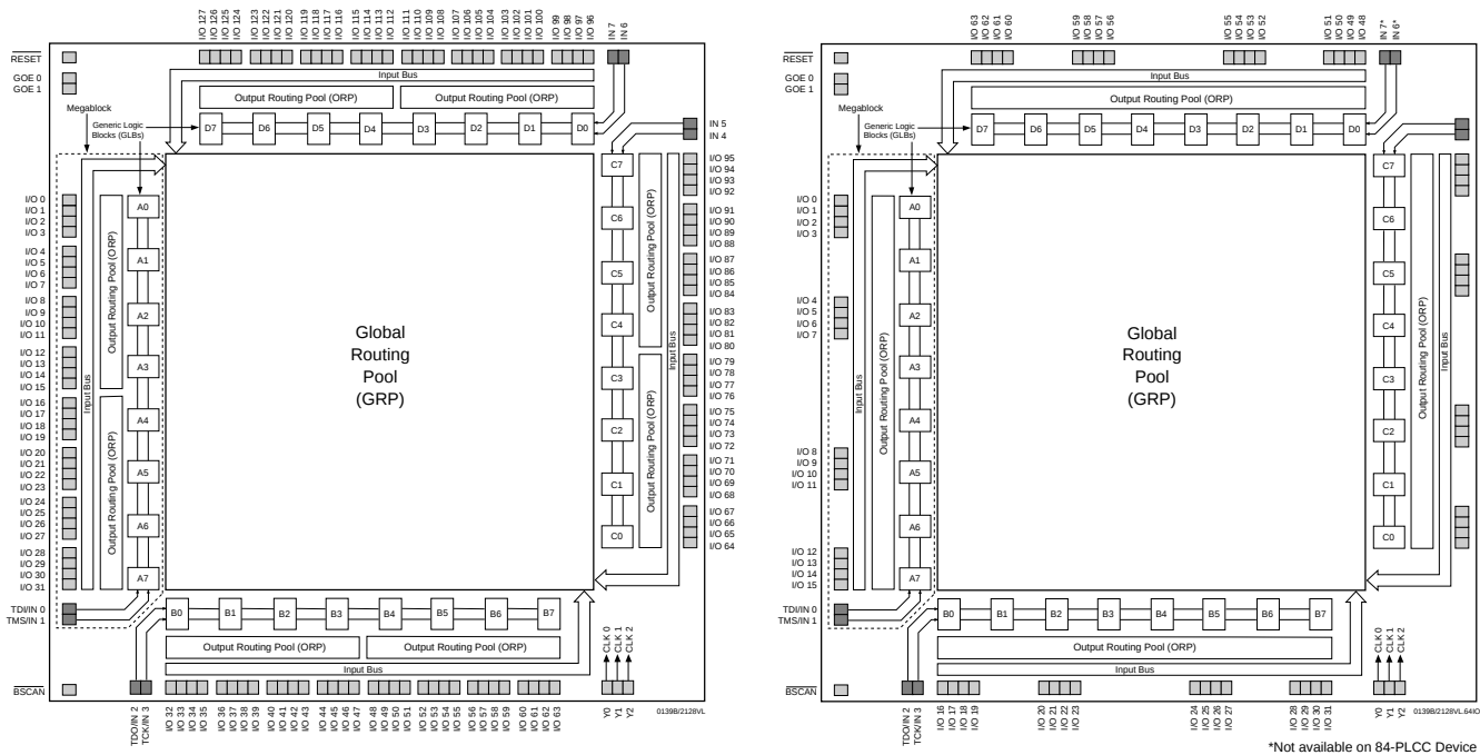
Figure 1. ispLSI 2128VL Functional Block Diagram (128-I/O and 64-I/O Versions)
