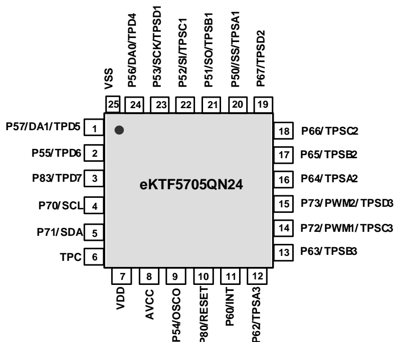
Figure 3-1 QFN-24 Pin Assignment
