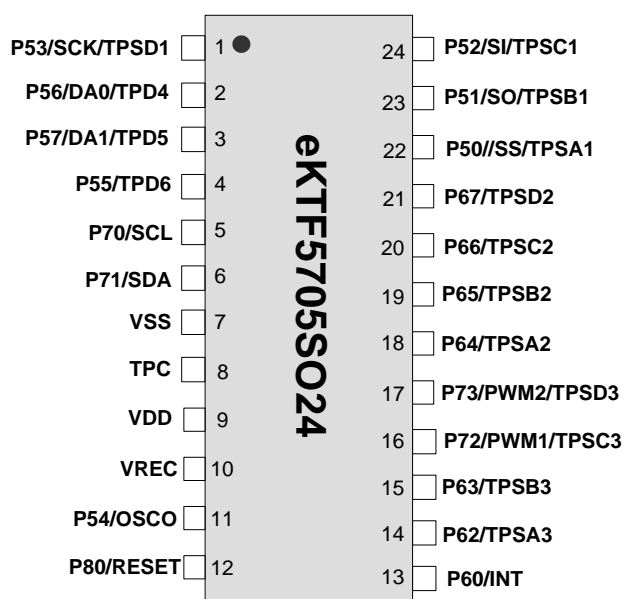
Figure 3-2 SOP-24 Pin Assignment
