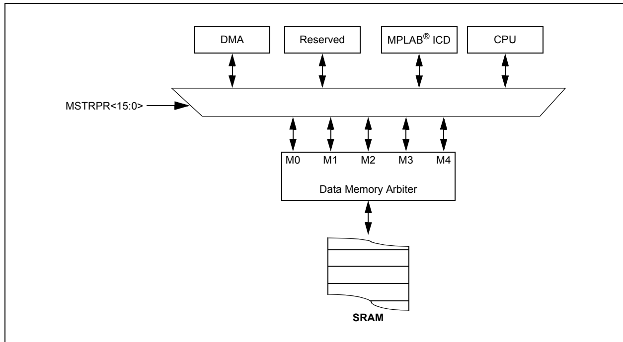
FIGURE 4-11: ARBITER ARCHITECTURE
