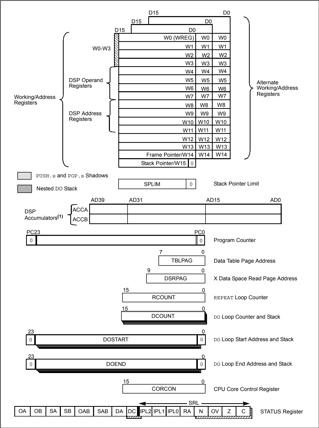
FIGURE 3-2: PROGRAMMER'S MODEL
