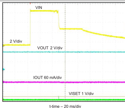
Figure 4. OVP 7-V Adaptor
