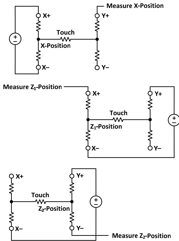
Figure 2: Pressure measurement block diagrams.
