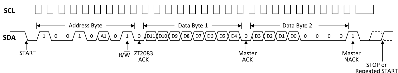
Figure 7: Complete I 2 C serial read transmission.
