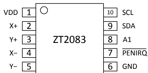
MSOP-10L Top View
