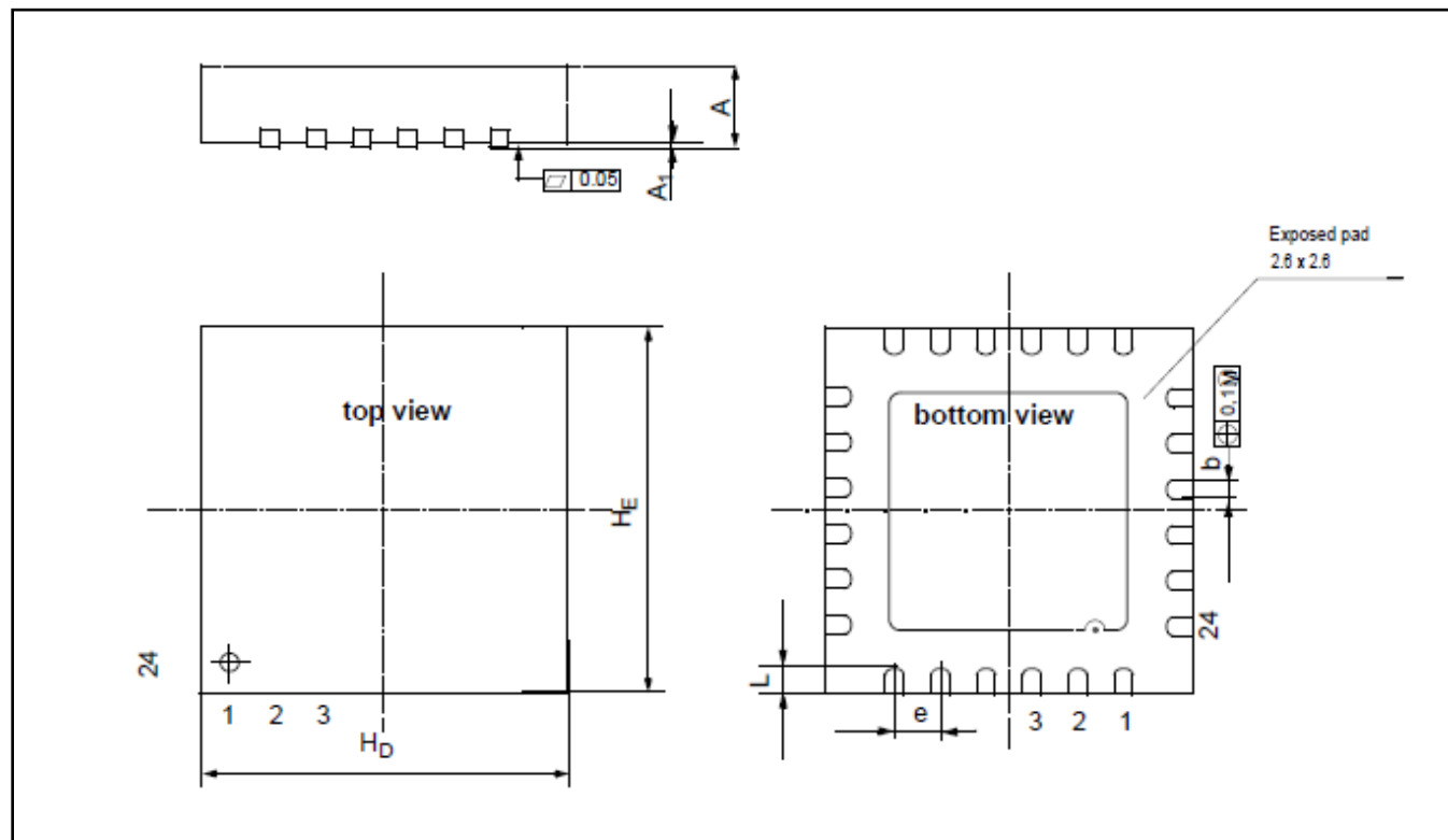
Figure 6.1 Package Drawing
