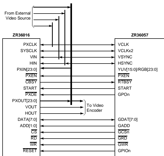
Figure 3. Recommended ZR36057 to ZR36016 Connections
