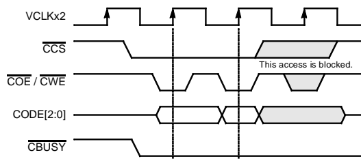
Figure 7. Transaction Termination
