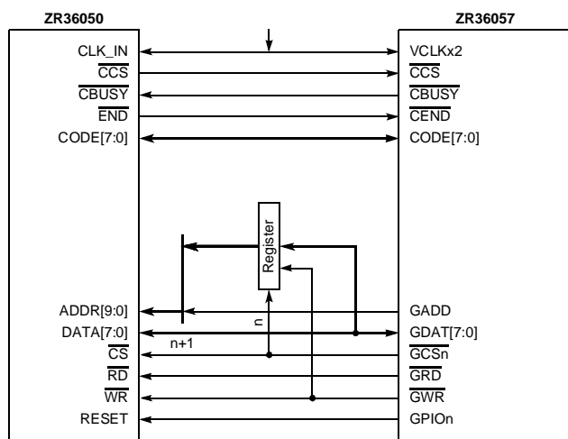
Figure 8. ZR36057 to ZR36050 Connections
