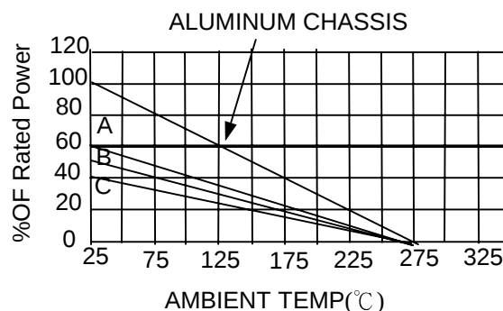
Derating Curve
