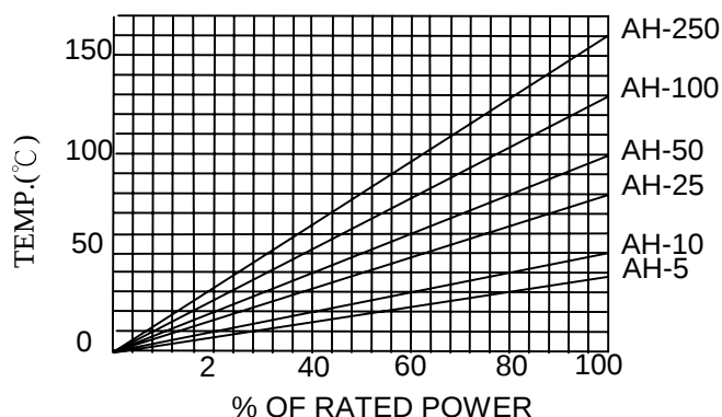
Surface Temperature Versus Power Load (On Chassis)
