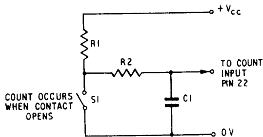
Fig. 3. Anti-Bounce Circuit
