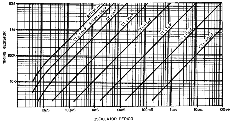
Fig. 4 Oscillator period
