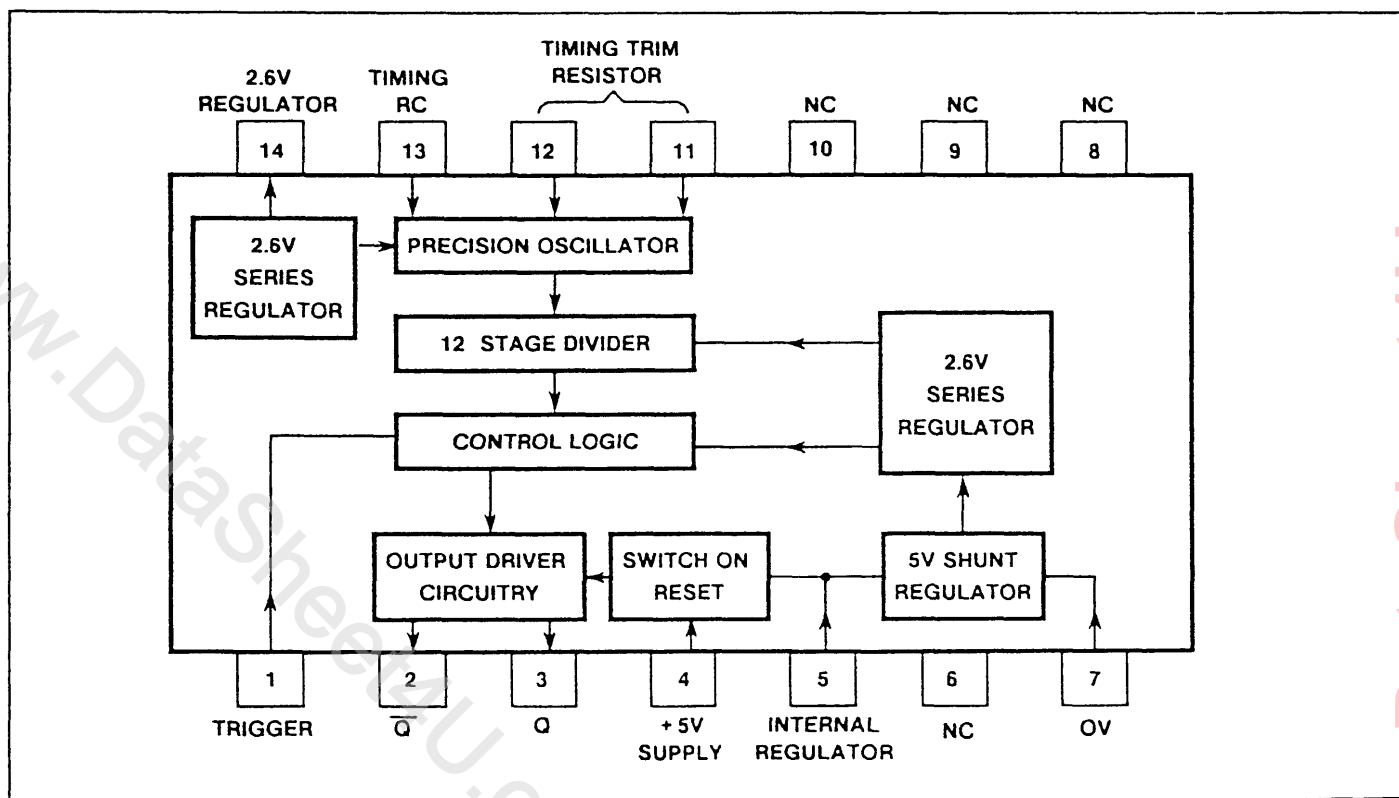
Fig.2 System diagram
