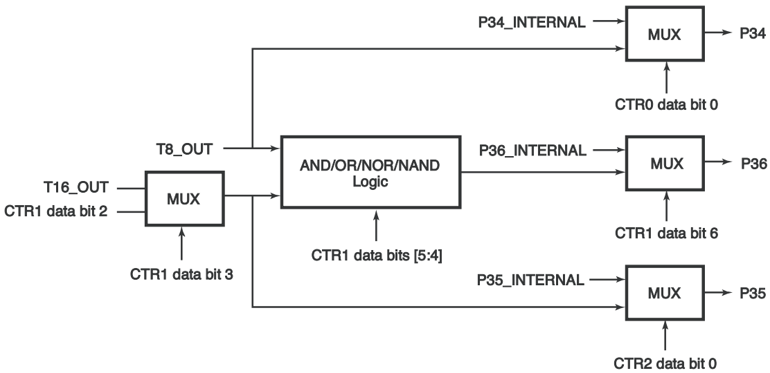
Figure 30. Output Circuit
