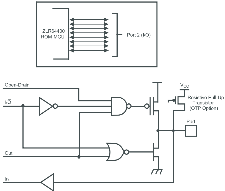
Figure 5. Port 2 Configuration
