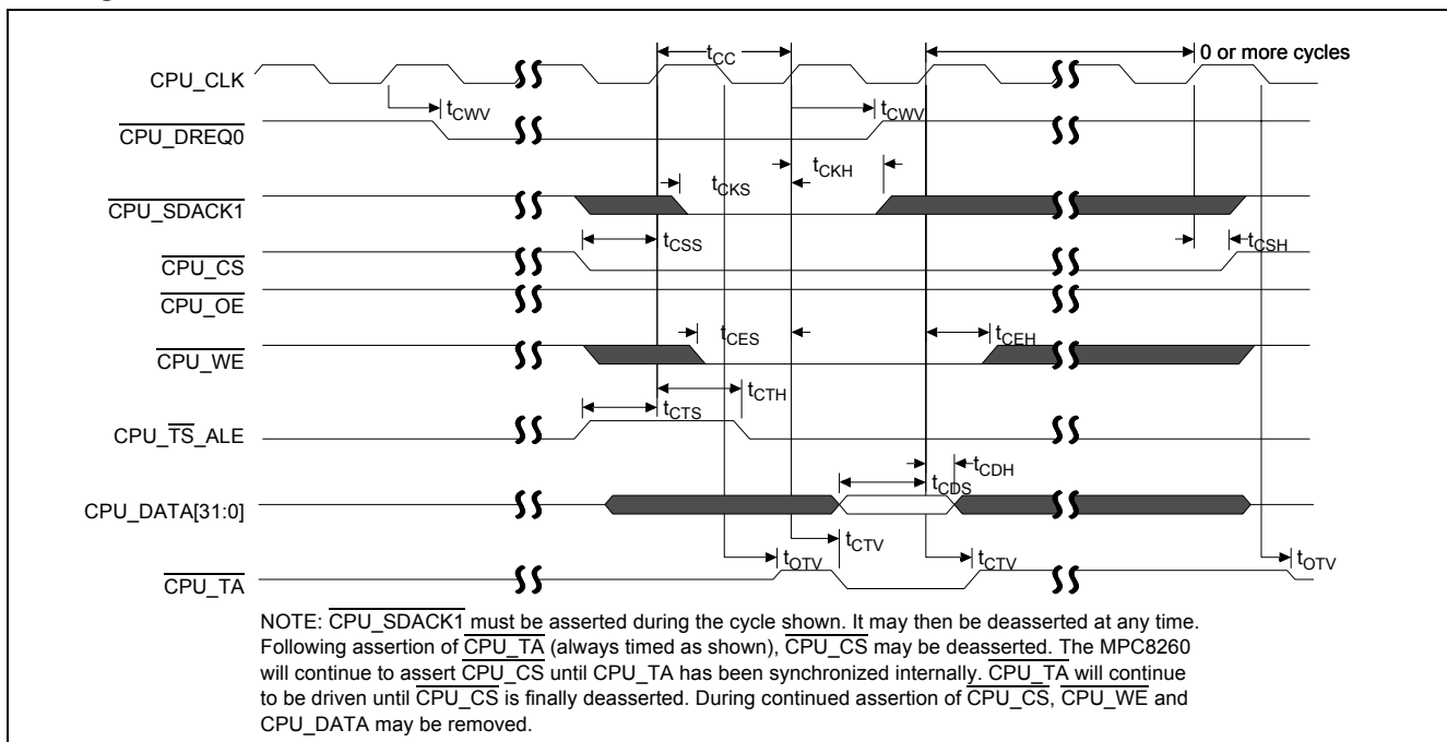
Figure 15 - CPU DMA Write
