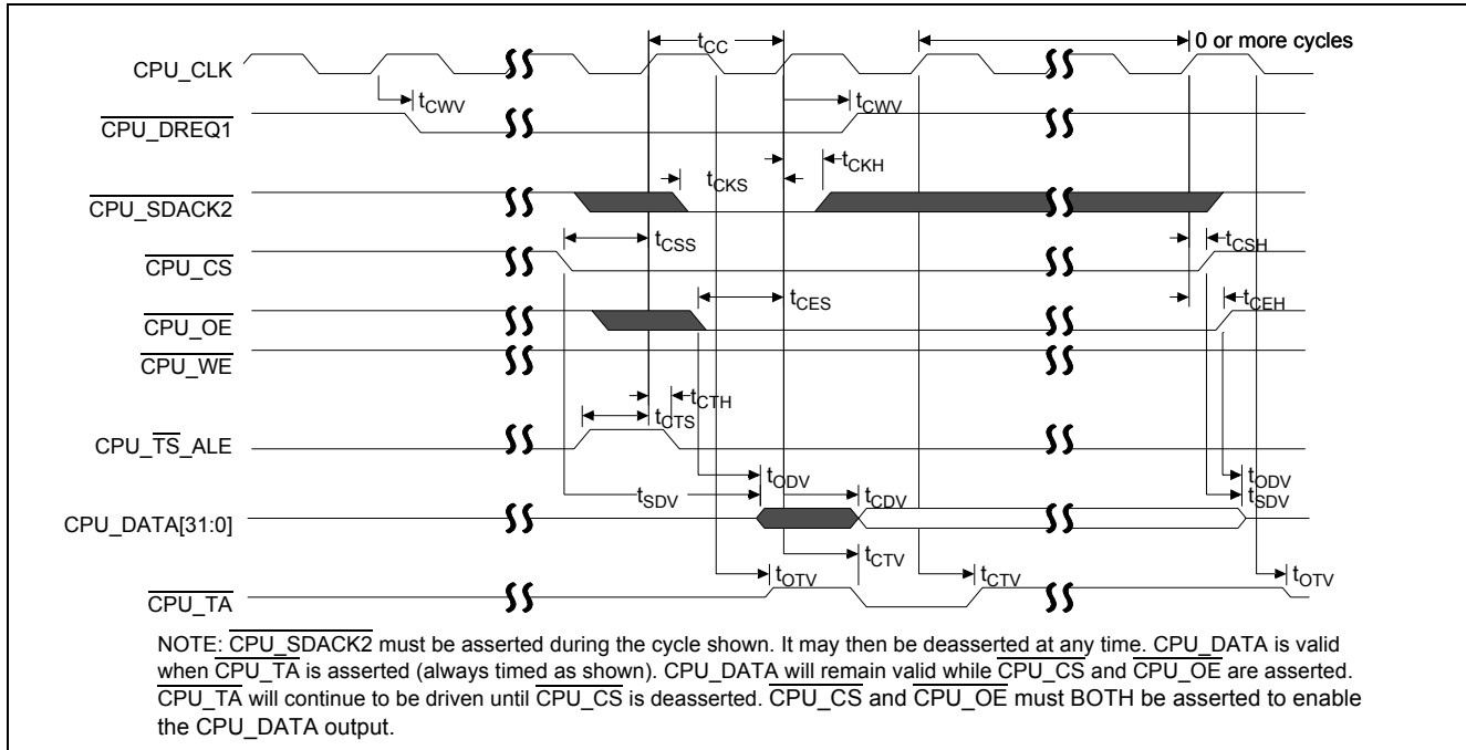
Figure 14 - CPU DMA Read
