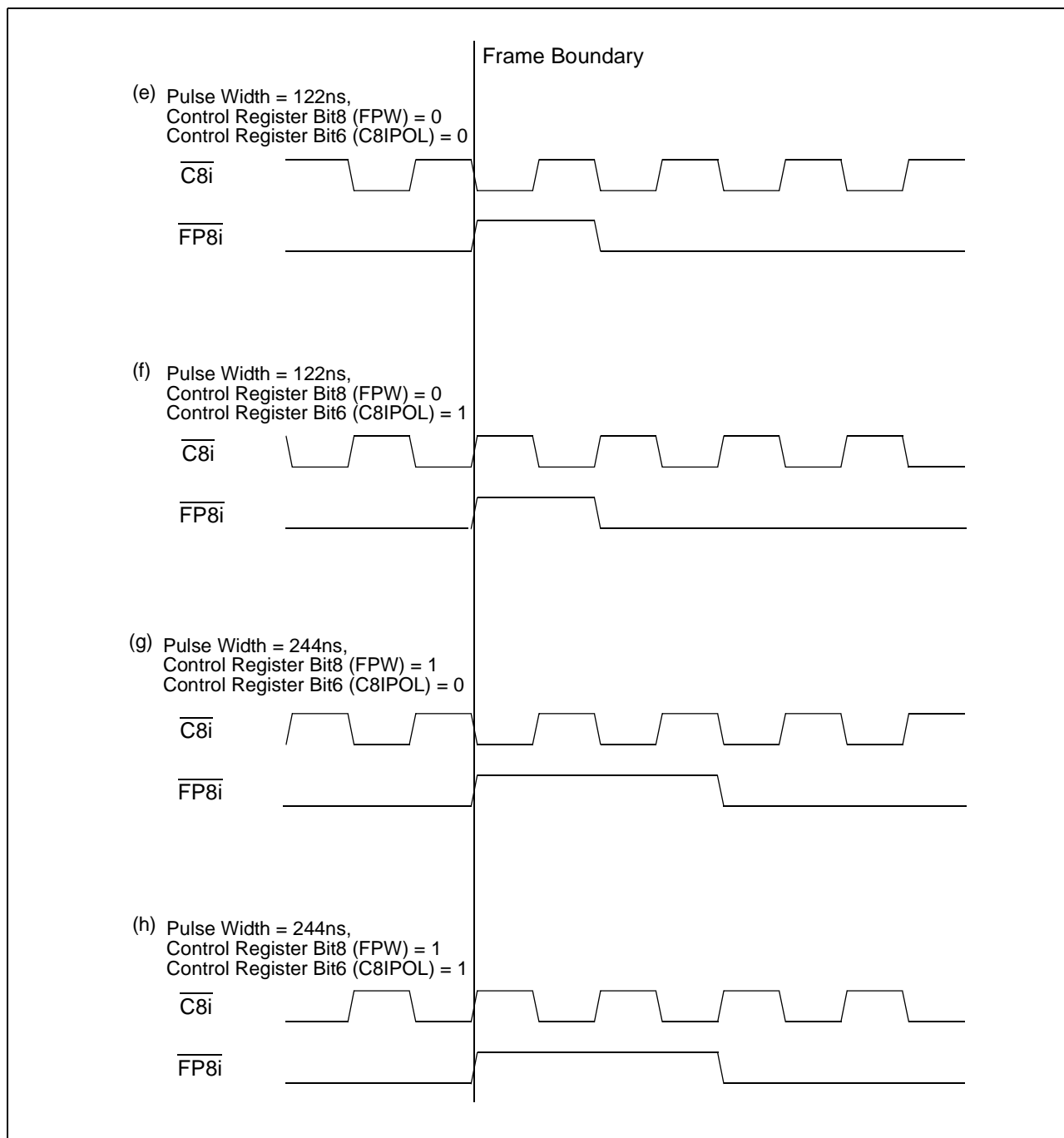
Figure 24 - Frame Boundary Conditions, GCI-Bus Operation
