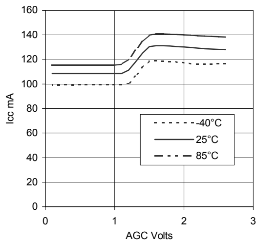
IS136 Tx. 1900 MHz - I_{cc} v AGC (Temperature)
