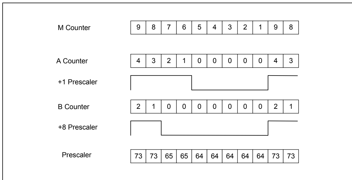
Figure 9 - Count Sequence for UHF PLL with 4 Modulus Prescaler
