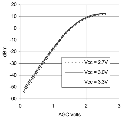
IS136 Tx. 900 MHz - Power Out v AGC ( V_{cc} )
