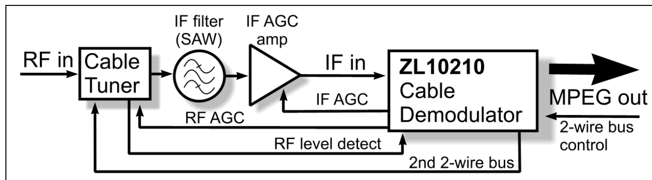
Figure 1 - System Diagram
