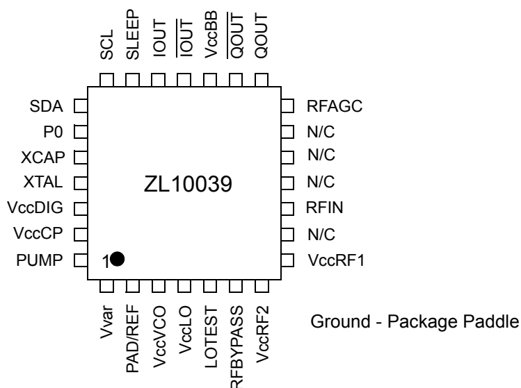
Figure 2 - Pin Diagram
