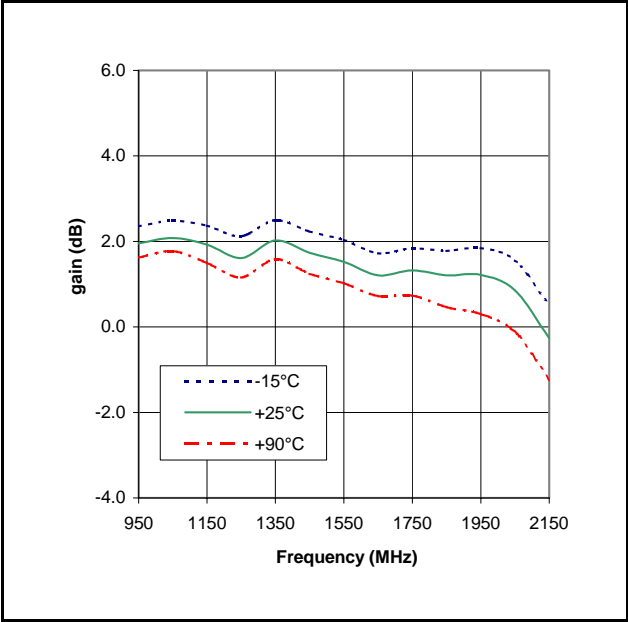
Figure 15 - RF Bypass Gain v Temperature
