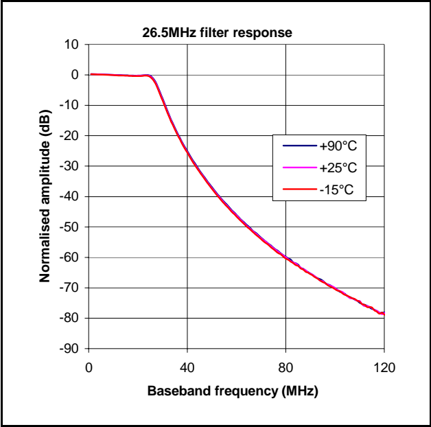
Figure 16 - Baseband Filter Response 26.5 MHz
