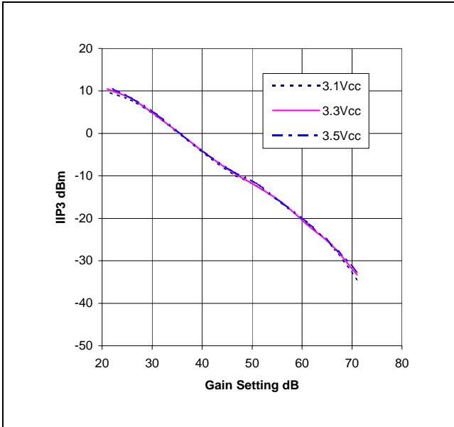
Figure 7 - IIP3 v Gain at 25°C
