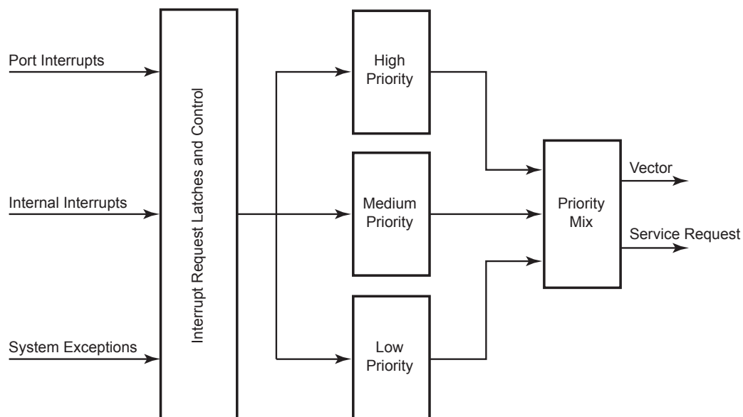
Figure 6. Interrupt Controller Block Diagram
