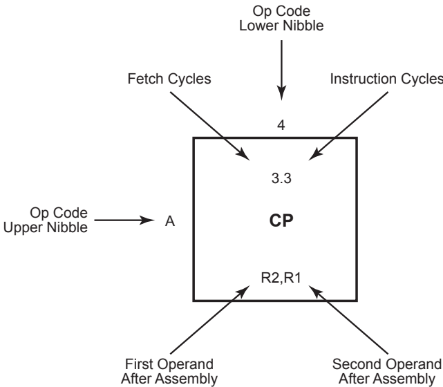
Figure 57. Op Code Map Cell Description
