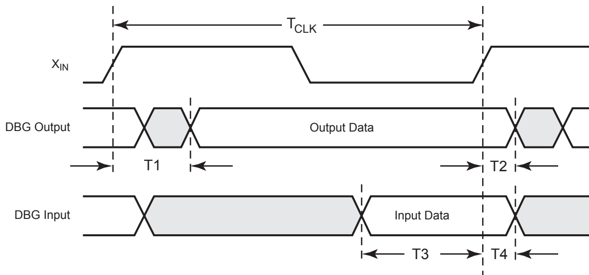
Figure 53. On-Chip Debugger Timing
