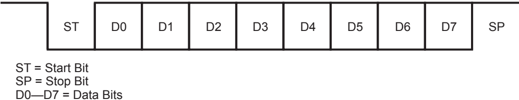
Figure 44. OCD Data Format
