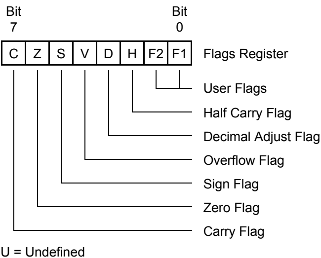
Figure 56. Flags Register
