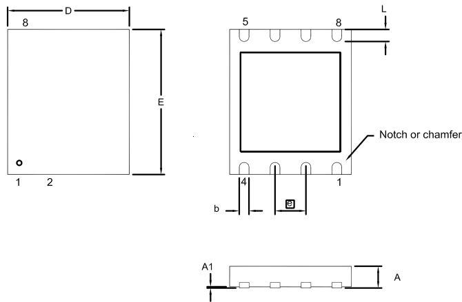
Figure 41.8-Pin Quad Flat No-Lead Package (QFN)/ MLF-S
