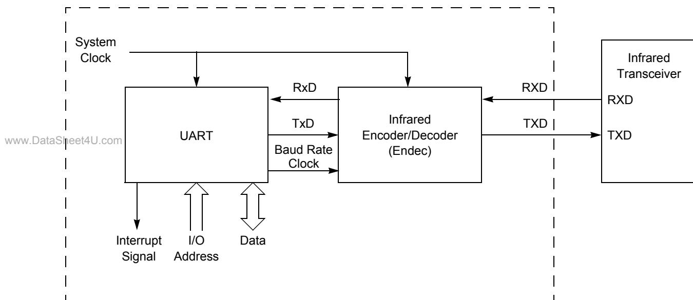
Figure 16. Infrared Data Communication System Block Diagram
