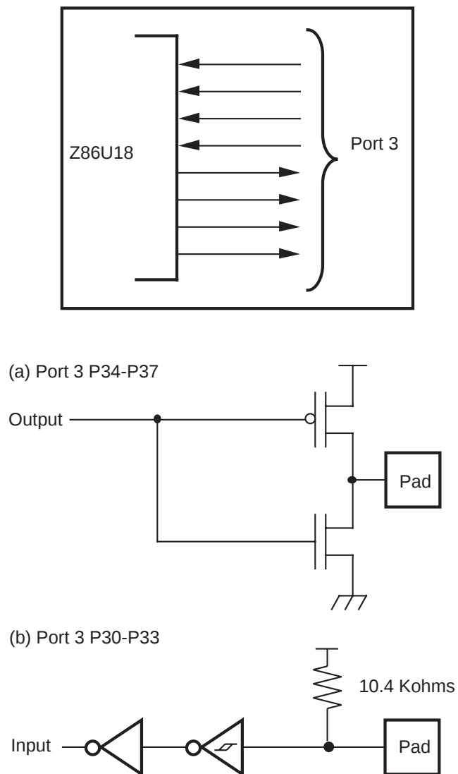
Figure 11. Port 3 Configuration
