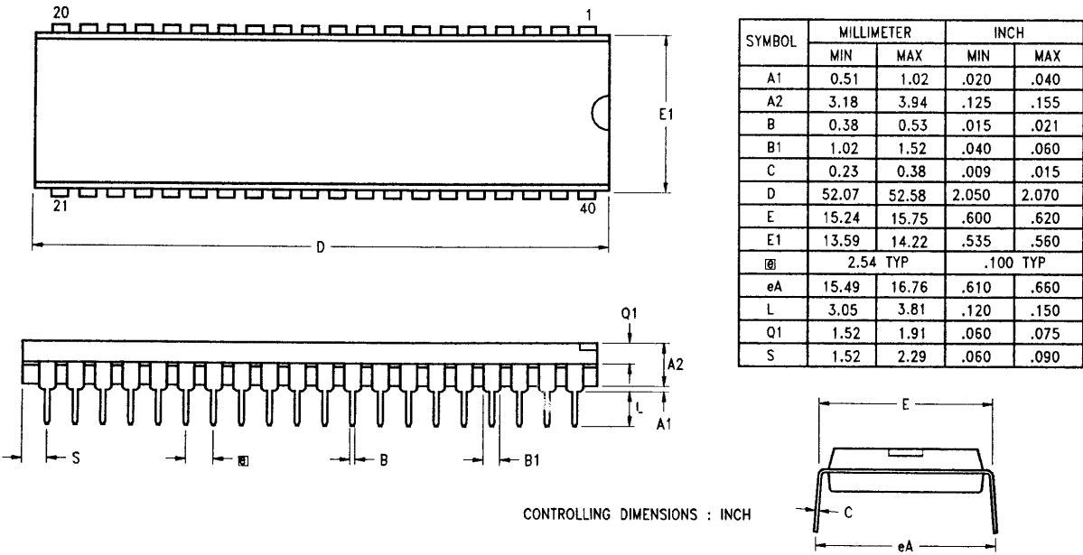
Figure 42. 40-Pin DIP
