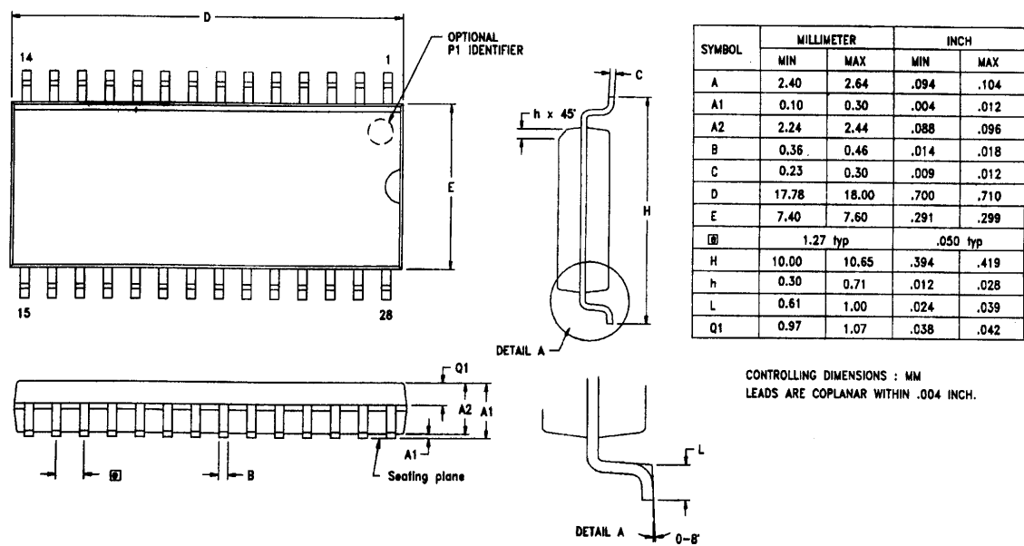
Figure 39. 28-Pin SOIC
