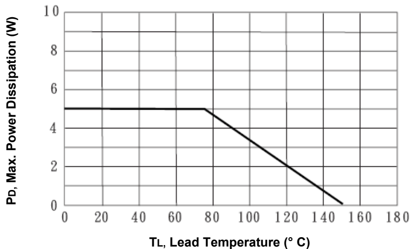
Fig.1-Power Temperature Derating Curve
