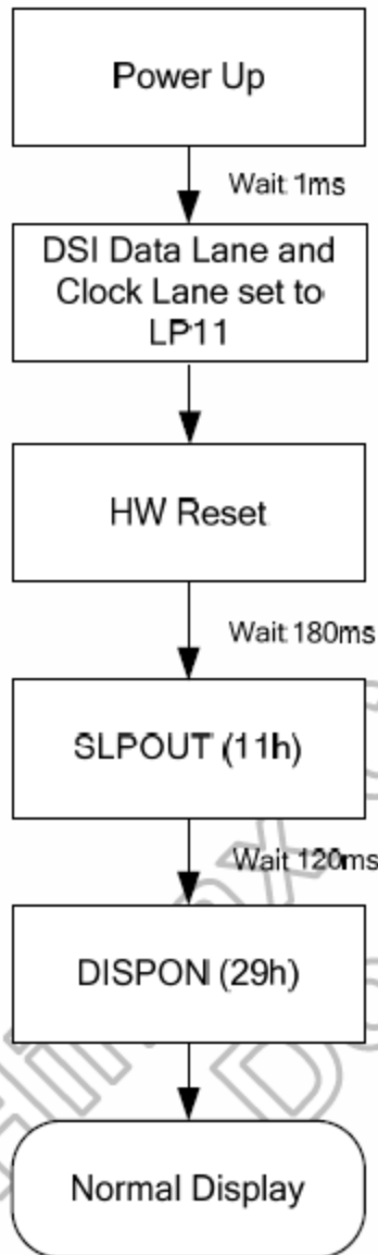
Power on/off sequence
