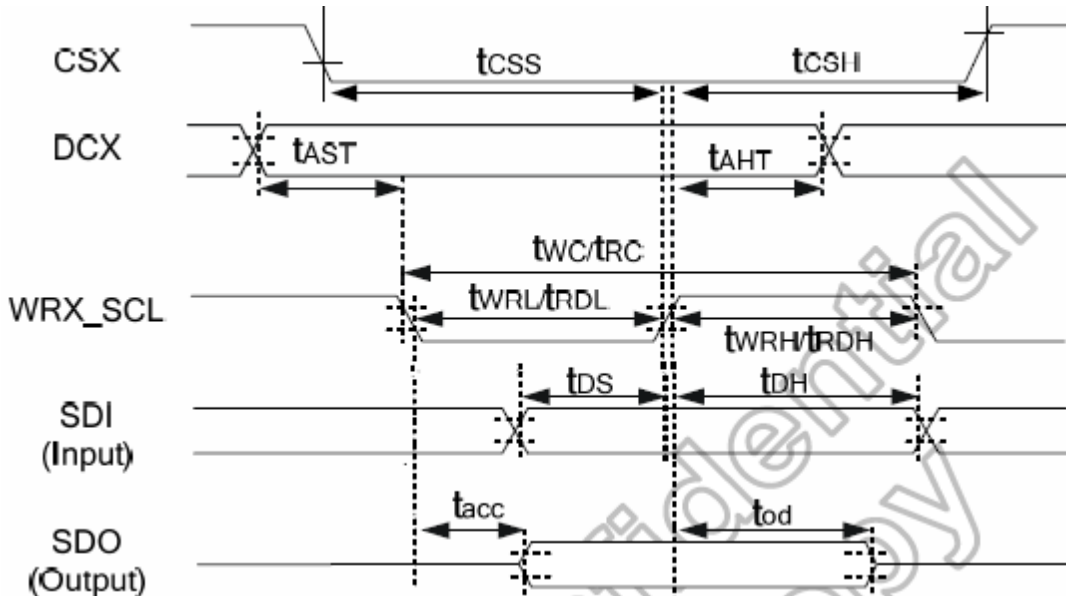
DBI Type C interface characteristics
