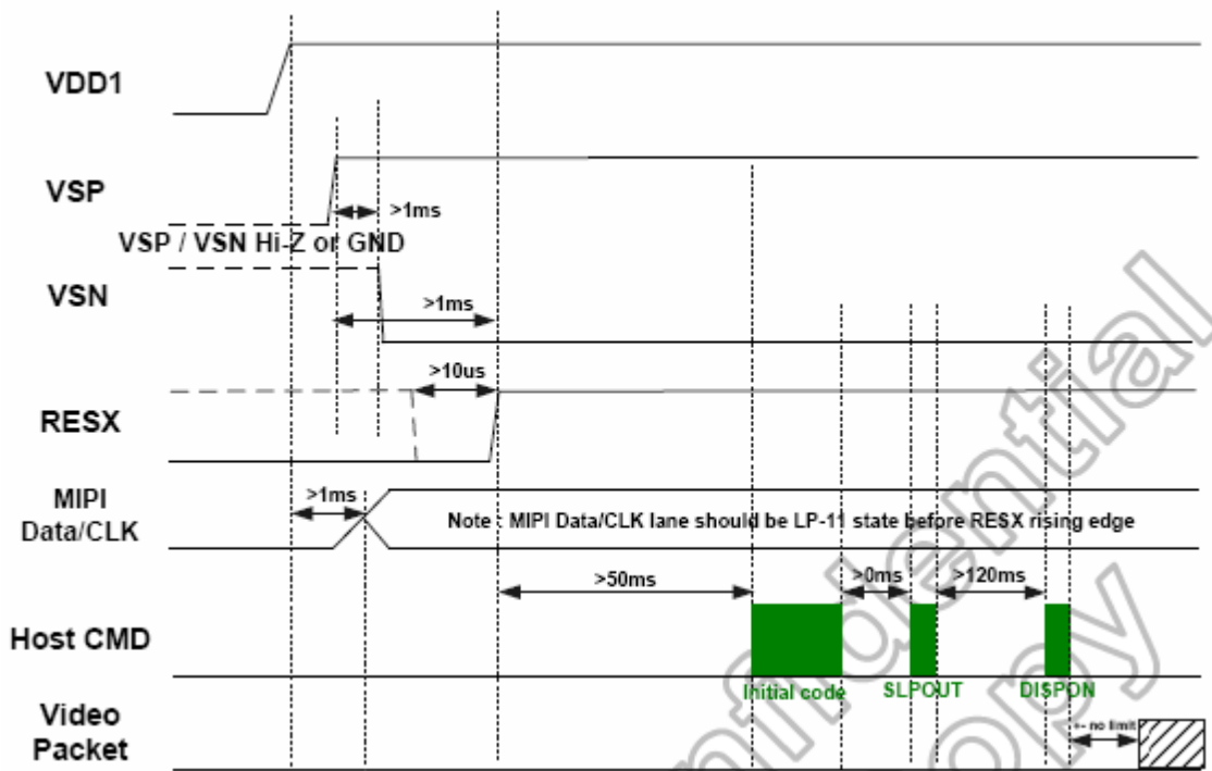
VDD1/ VSP/VSN input power on sequence
