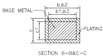
SECTION B-B&C-C
