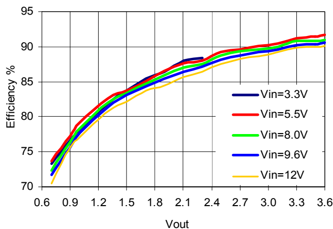
Figure 4. Efficiency Vs. Output Voltage at Iout=17A and Different Input Voltages
