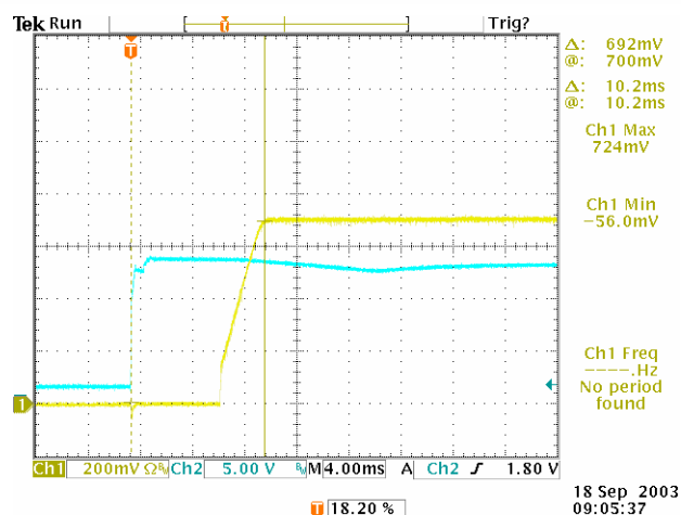
Figure 8. V_{in}=13.2V , V_{out}=0.7V , I_{out}=8.5A . Ch1 – V_{out} , Ch2 – V_{in}
