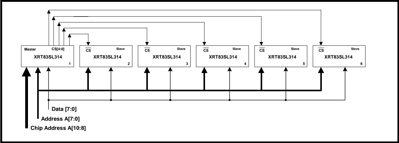
FIGURE 32. SIMPLIFIED BLOCK DIAGRAM OF AN 84-CHANNEL APPLICATION
