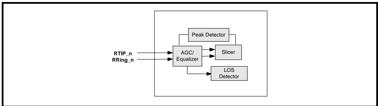
FIGURE 7. AGC/EQUALIZER BLOCK DIAGRAM
