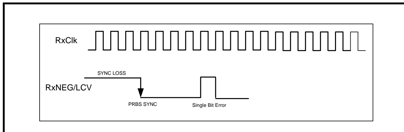
FIGURE 29. PRBS MODE
