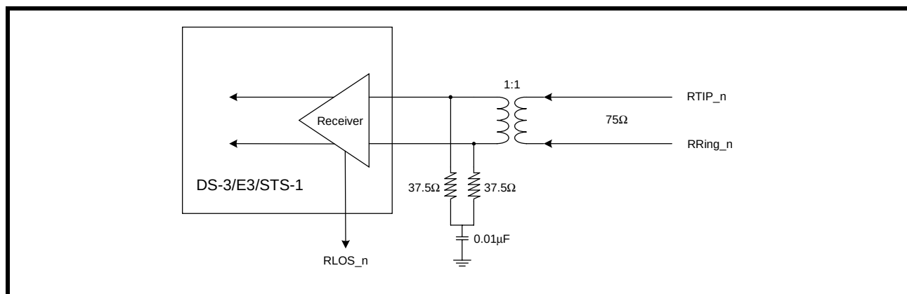
FIGURE 19. RECEIVE LINE INTERFACE CONNECTION
