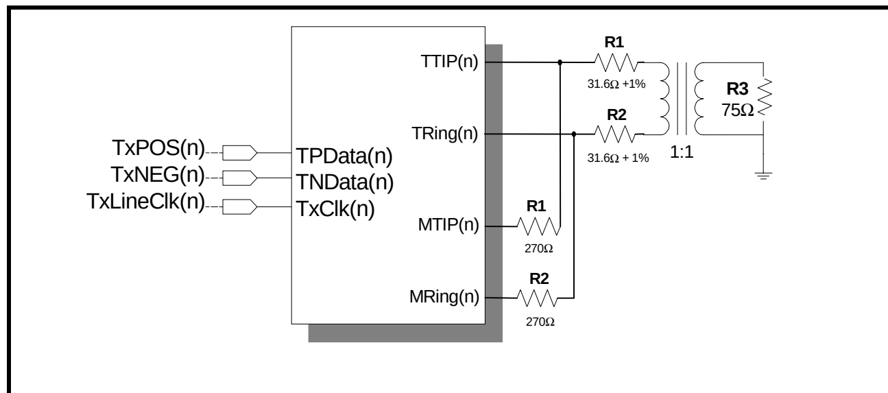
FIGURE 17. TRANSMIT DRIVER MONITOR SET-UP.
