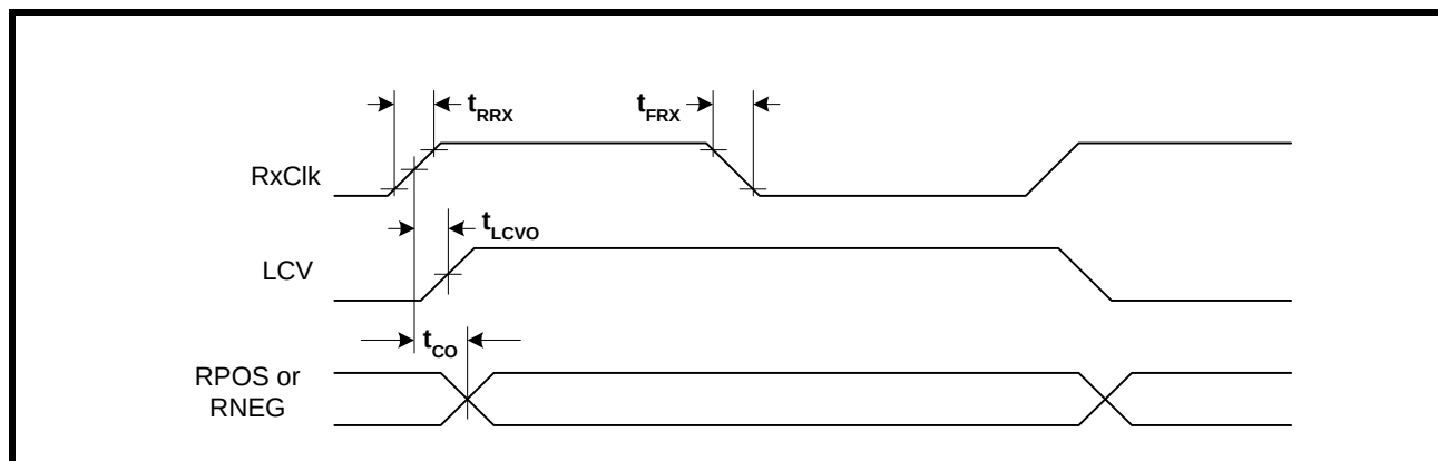
FIGURE 25. RECEIVER DATA OUTPUT AND CODE VIOLATION TIMING
