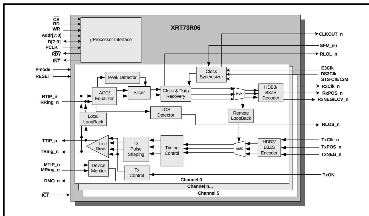
FIGURE 1. BLOCK DIAGRAM OF THE XRT 73R06
