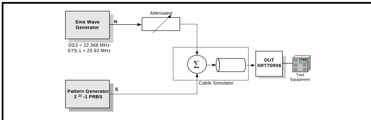
FIGURE 23. INTERFERENCE MARGIN TEST SET UP FOR DS3/STS-1
