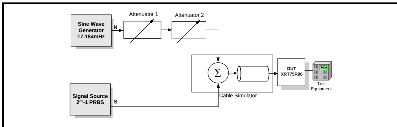
FIGURE 24. INTERFERENCE MARGIN TEST SET UP FOR E3.
