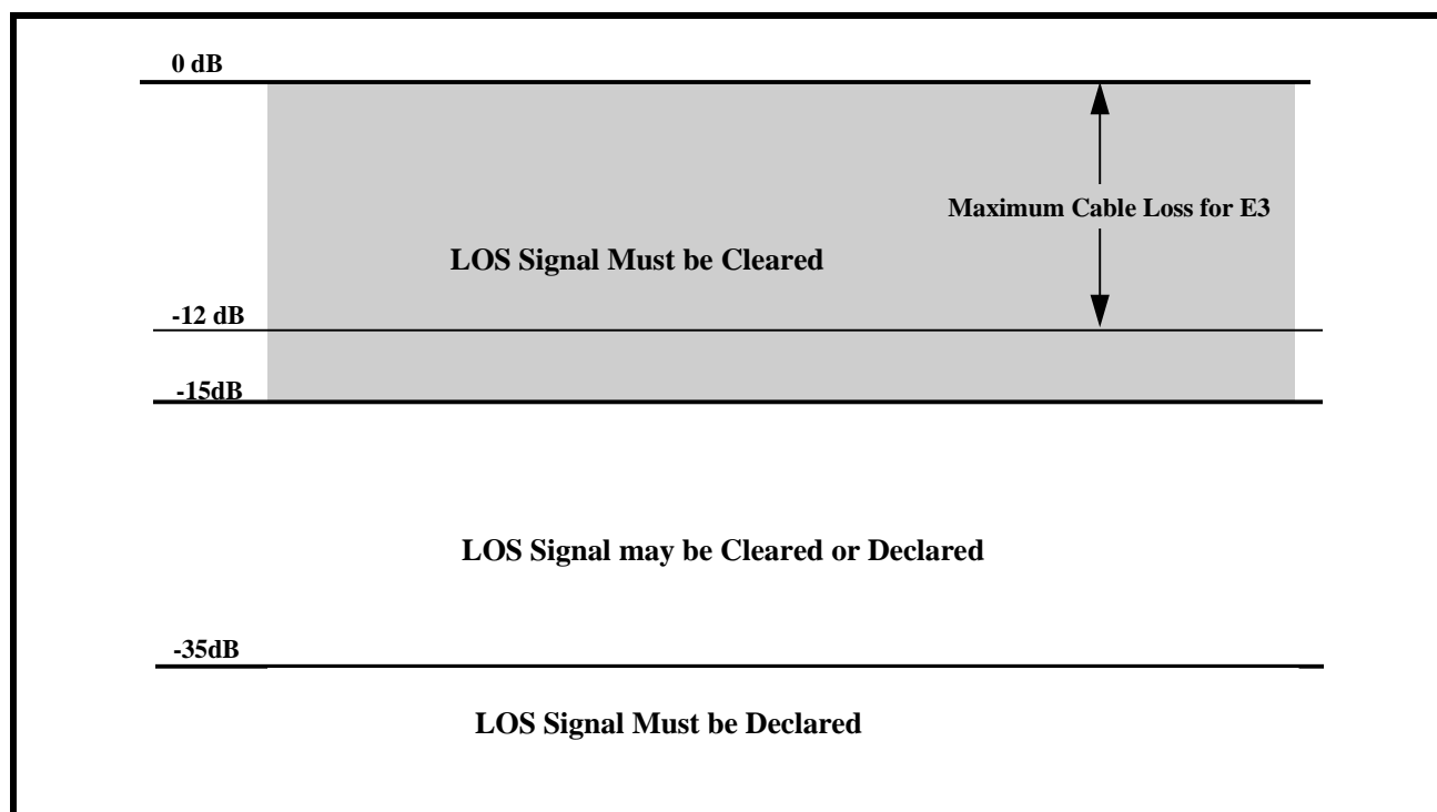
FIGURE 22. THE SIGNAL LEVELS THAT THE XRT73LC00 DECLARES AND CLEARS LOS (E3 MODE ONLY)
