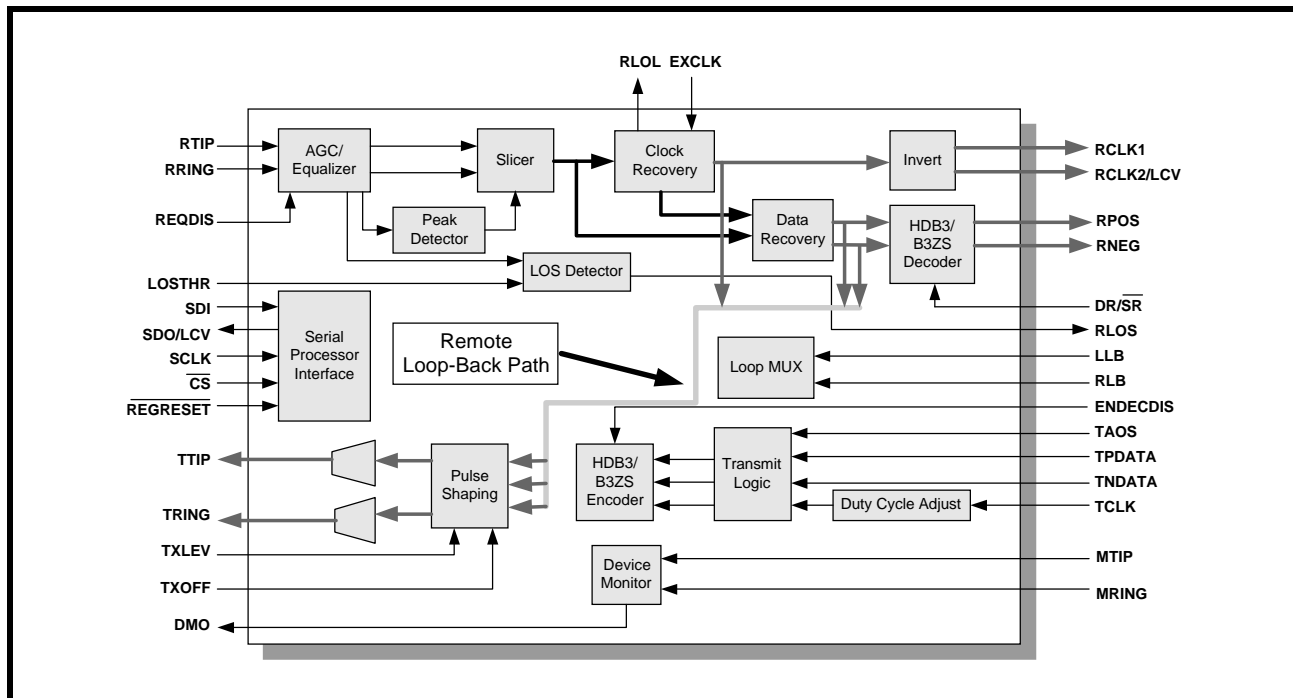
FIGURE 31. THE REMOTE LOOP-BACK PATH IN THE XRT73LC00
