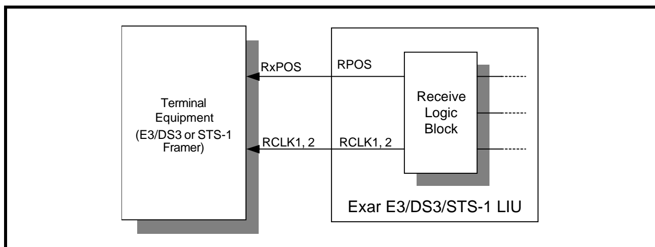
FIGURE 27. THE TYPICAL INTERFACE FOR THE TRANSMISSION OF DATA IN A SINGLE-RAIL FORMAT FROM THE RECEIVE SECTION OF THE XRT73LC00 TO THE RECEIVING TERMINAL EQUIPMENT
