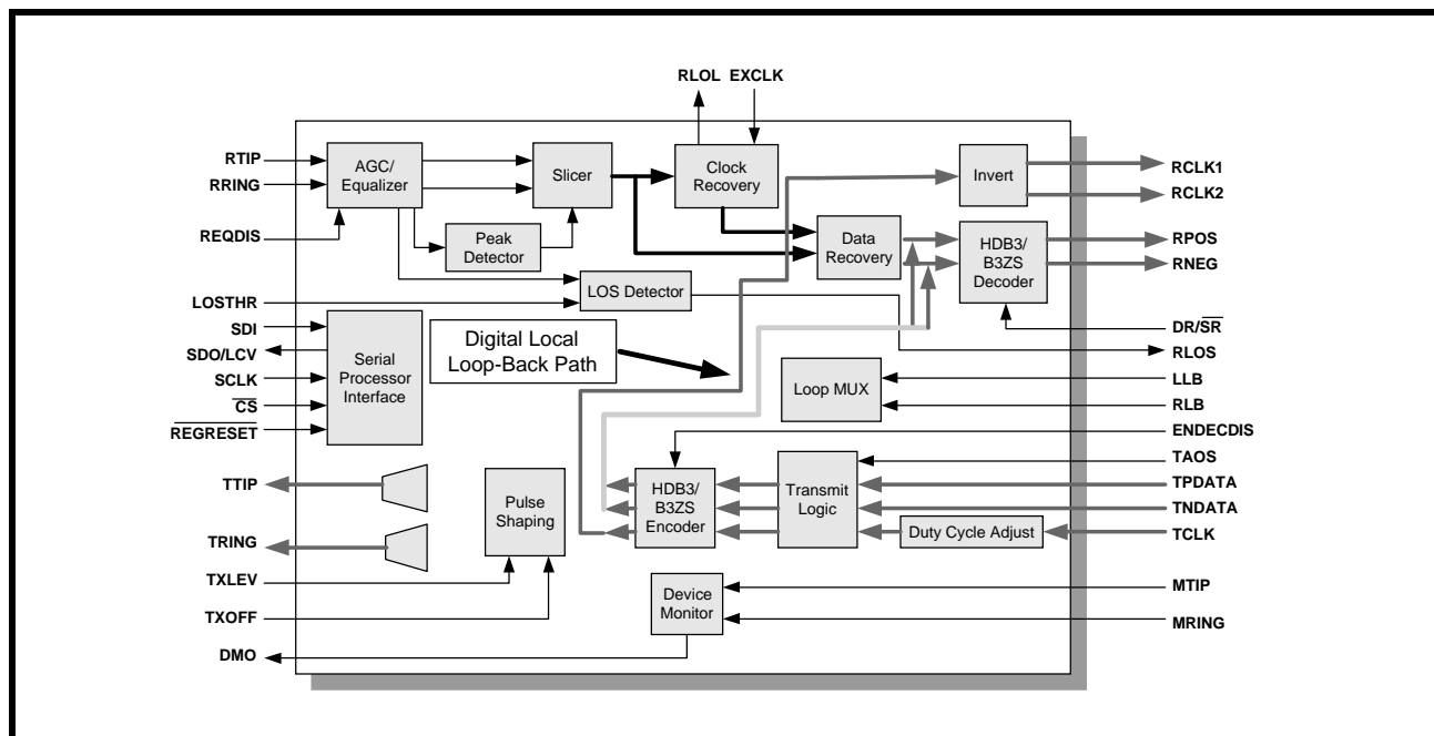
FIGURE 30. THE DIGITAL LOCAL LOOP-BACK PATH IN THE XRT73LC00
