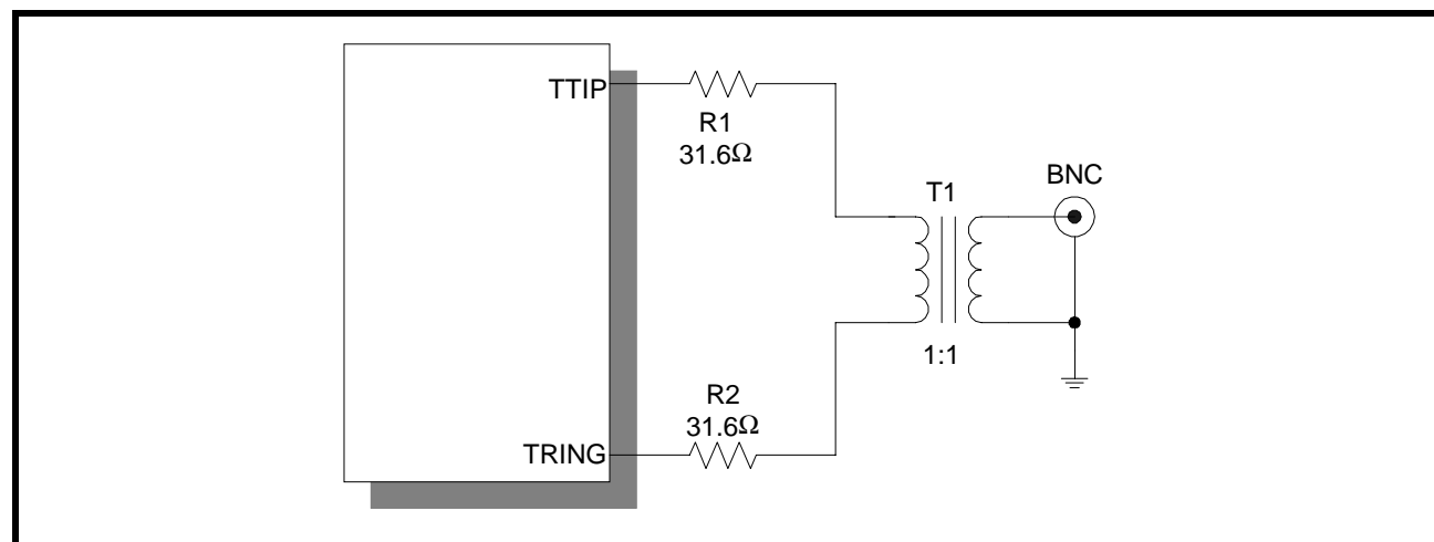
FIGURE 16. RECOMMENDED SCHEMATIC FOR INTERFACING THE TRANSMIT SECTION OF THE XRT73LC00 TO THE LINE
