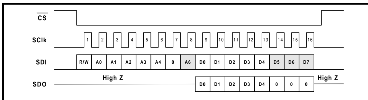
FIGURE 33. MICROPROCESSOR SERIAL INTERFACE DATA STRUCTURE
