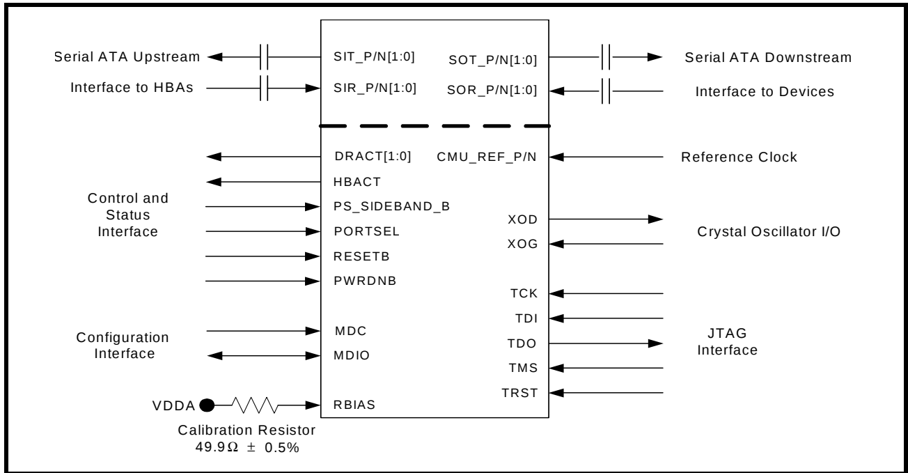
FIGURE 3. XRS10L220 INTERFACES
