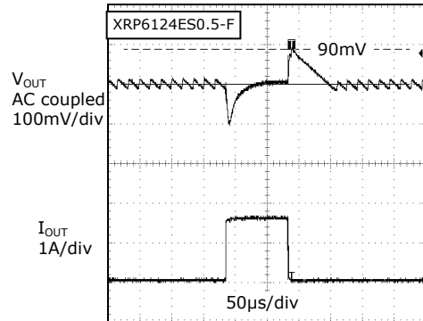
Fig. 16: Load step transient response corresponding to a CCM-DCM transition, 0.05A-1.6A-0.05A
