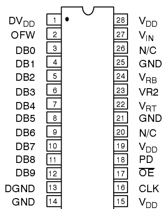
28 Lead PDIP (0.300")
