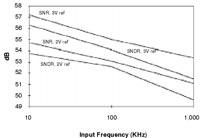
Figure 13. XRD64L15 SNR & SNDR vs. F_{IN} , V_{DD} = 3.3V , DV_{DD} = 3.3V , V_{REF} = 3V \text{ \& } 2V , F_S = 20MSPS , C_{IN} = 100pF
