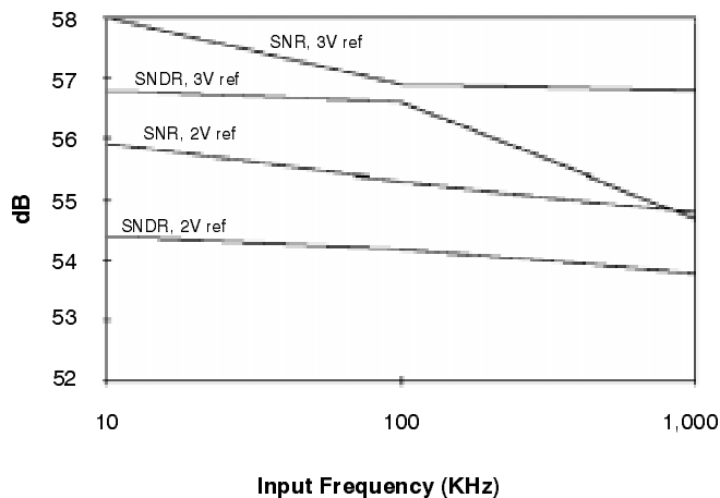
Figure 12. XRD64L15 SNR & SNDR vs. F_{IN} , V_{DD} = 3.3V , DV_{DD} = 3.3V , V_{REF} = 3V \text{ \& } 2V , F_S = 15MSPS , C_{IN} = 100pF
