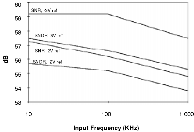
Figure 10. XRD64L15 SNR & SNDR vs. F_{IN} , V_{DD} = 3.3V , DV_{DD} = 3.3V , V_{REF} = 3V \text{ \& } 2V , F_S = 10MSPS , C_{IN} = 100pF
