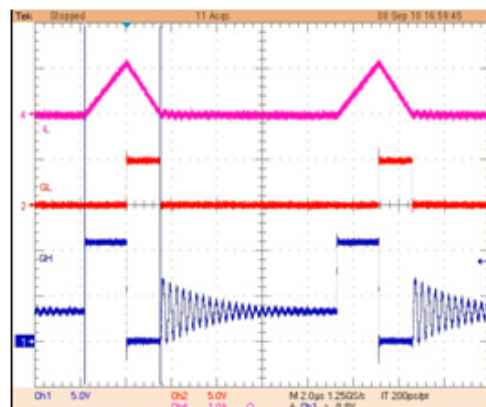
Figure 3: 0-6A Transient 300kHz PWM only
