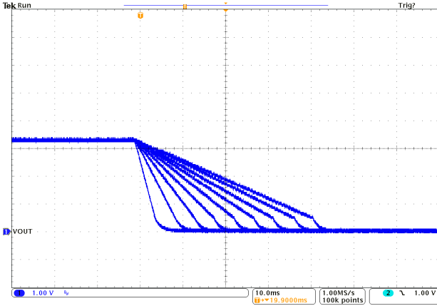
Figure 10: Simultaneous Shut-Down
