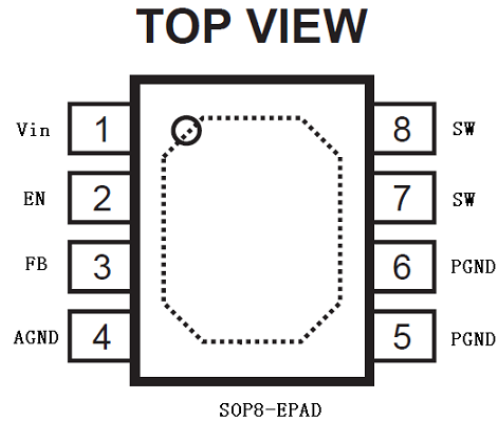
Figure 2. PIN Configuration
