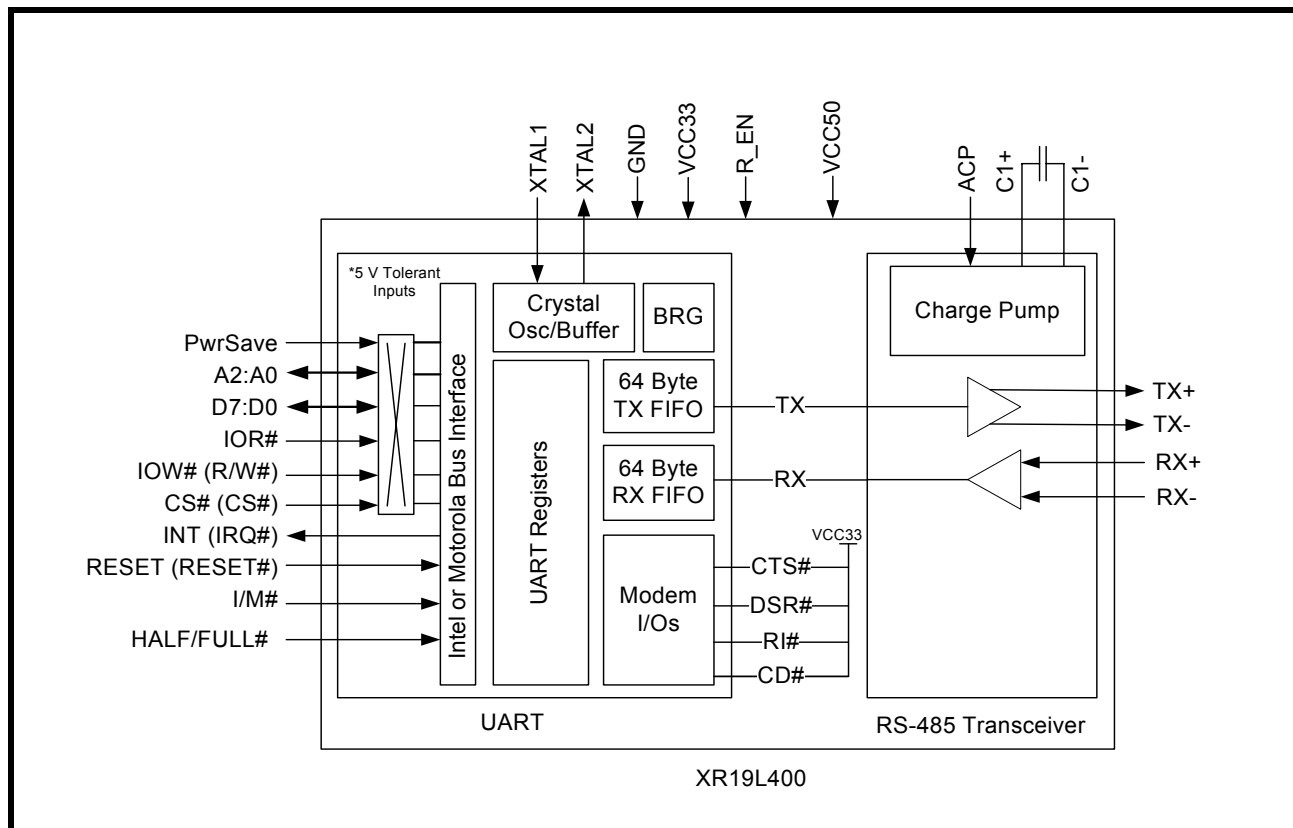
FIGURE 1. BLOCK DIAGRAM
