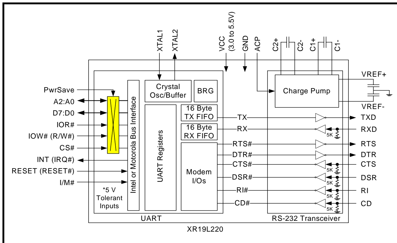
FIGURE 1. BLOCK DIAGRAM
