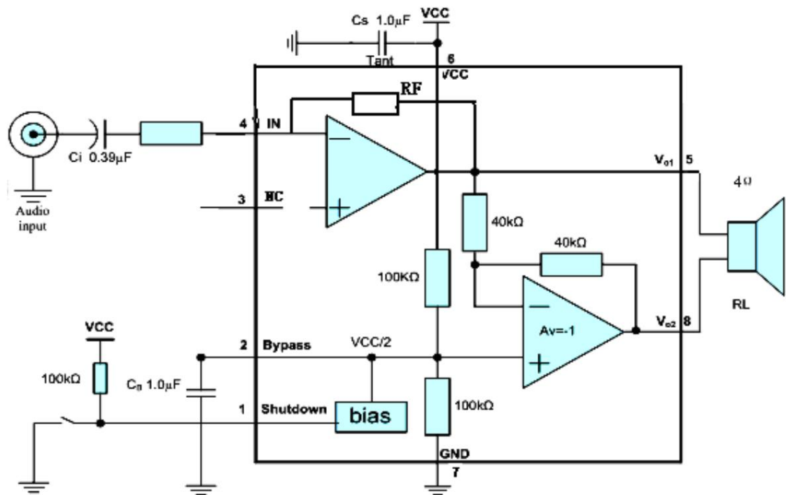
Figure 1 XPT6871 typical application circuit
