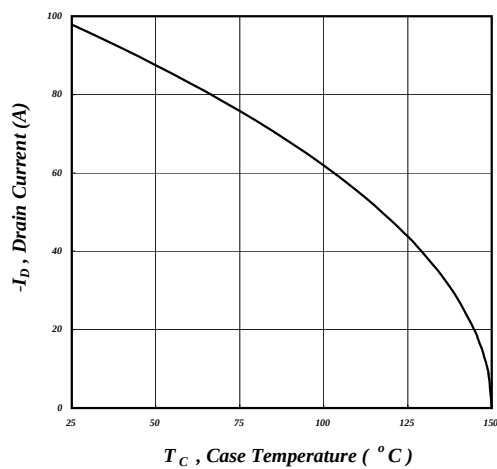
Fig 11. Drain Current v.s. Case Temperature
