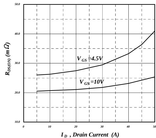
Fig 6. Typ. Drain-Source on State Resistance
