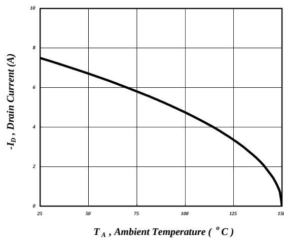
Fig 12. Drain Current v.s. Ambient Temperature
