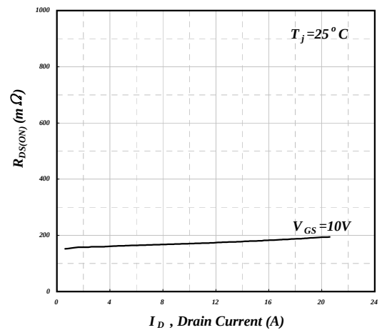
Fig 12. Typ. Drain-Source on State Resistance
